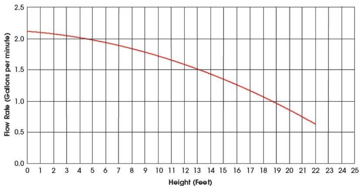
CP-22 Pump Performance Curve
