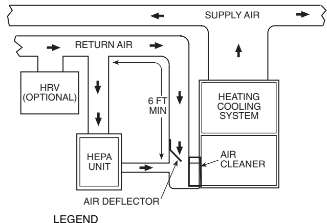
Fig. 3 — Typical Air Cleaner Installation
