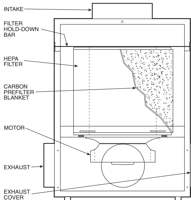
Fig. 2 — Filter Installation
