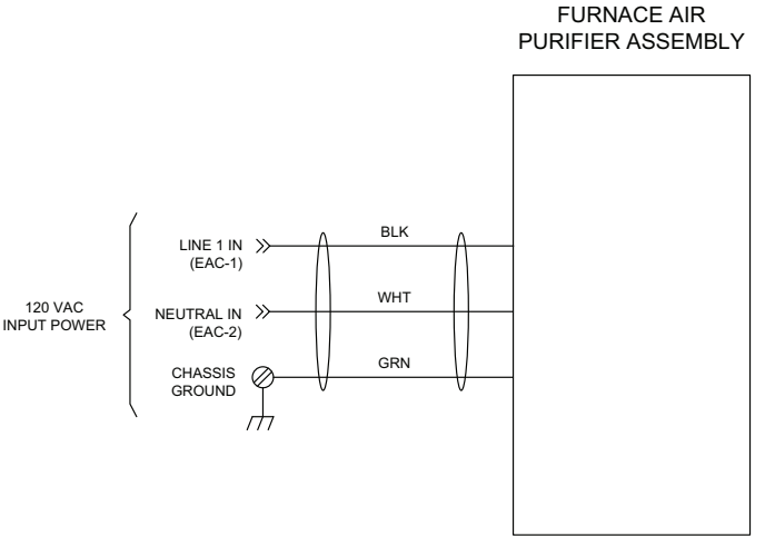
Fig. 11 – Furnace Installation
