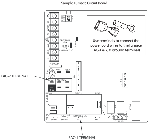
Fig. 12 – Air Purifier Connection to Furnace
