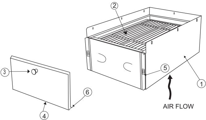
Fig. 2 – FNCCAB Major Components
