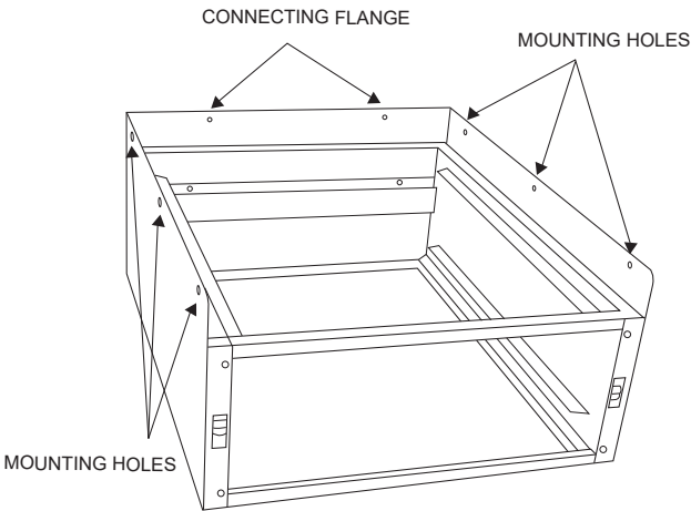
Fig. 5 – Mounting Holes and Mounting Flange
