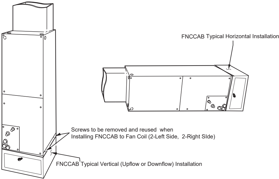
Fig. 4 – Typical Installation
