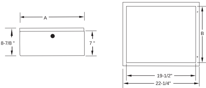
Fig. 3 – FNCCAB Dimensions
