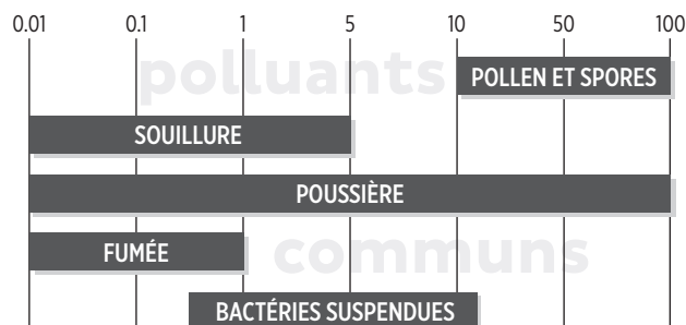
FIGURE 2 – POLLUANTS COMMUNS
