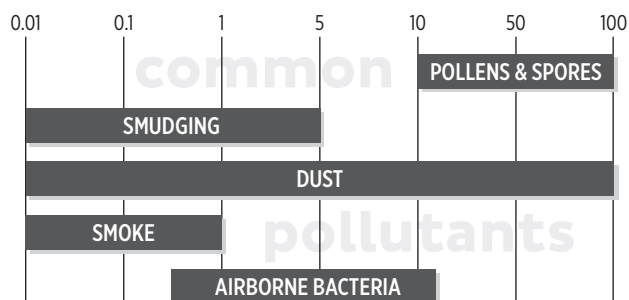
FIGURE 2 – COMMON POLLUTANTS
