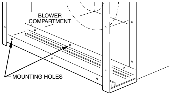
Fig. 7 – Mounting Holes
