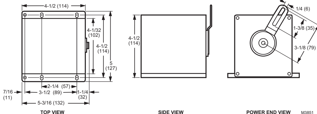
Fig. 1. M7215 Damper Motor dimensions in in. (mm).
