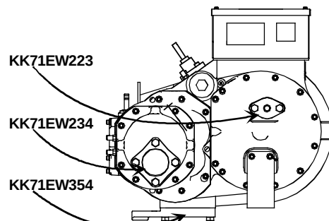
TYPICAL COMPRESSOR
