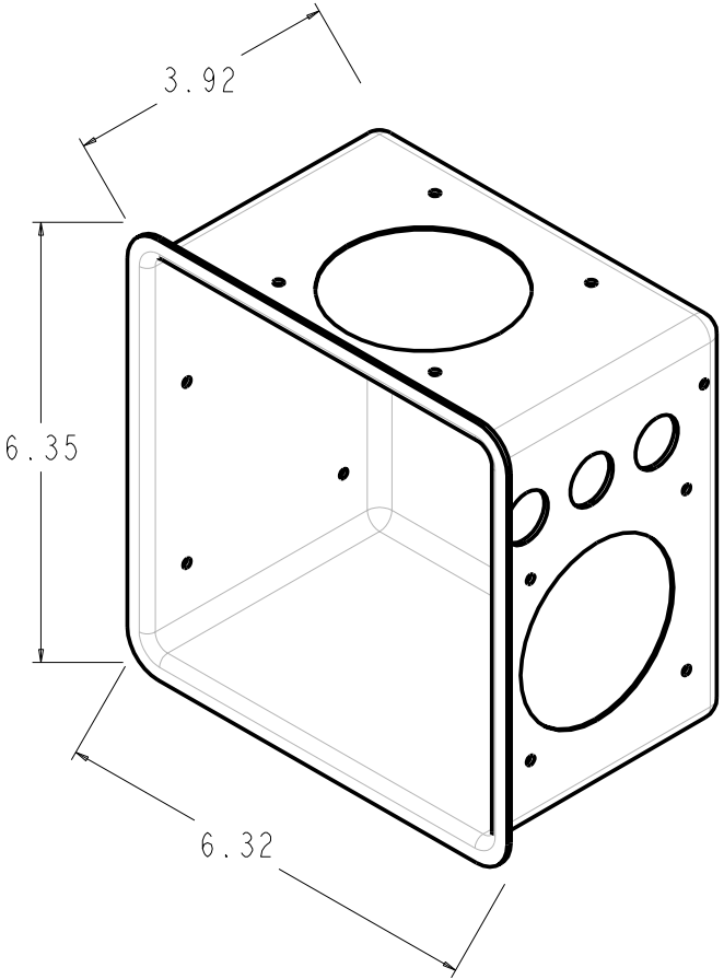
ELECTRICAL BOX
