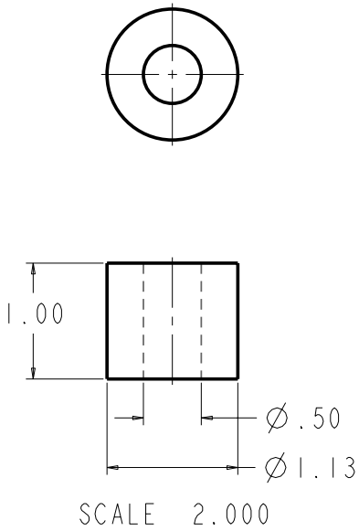
SOLID MOUNT 30HR070_1071
