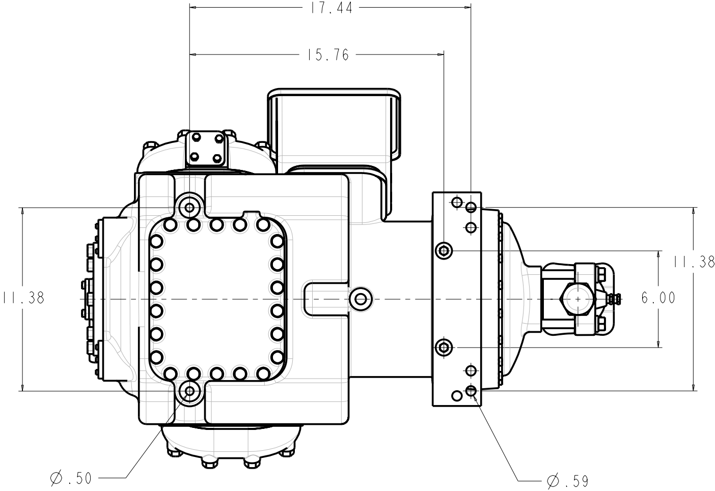
BOTTOM VIEW MOUNTING BOLT PATTERN
