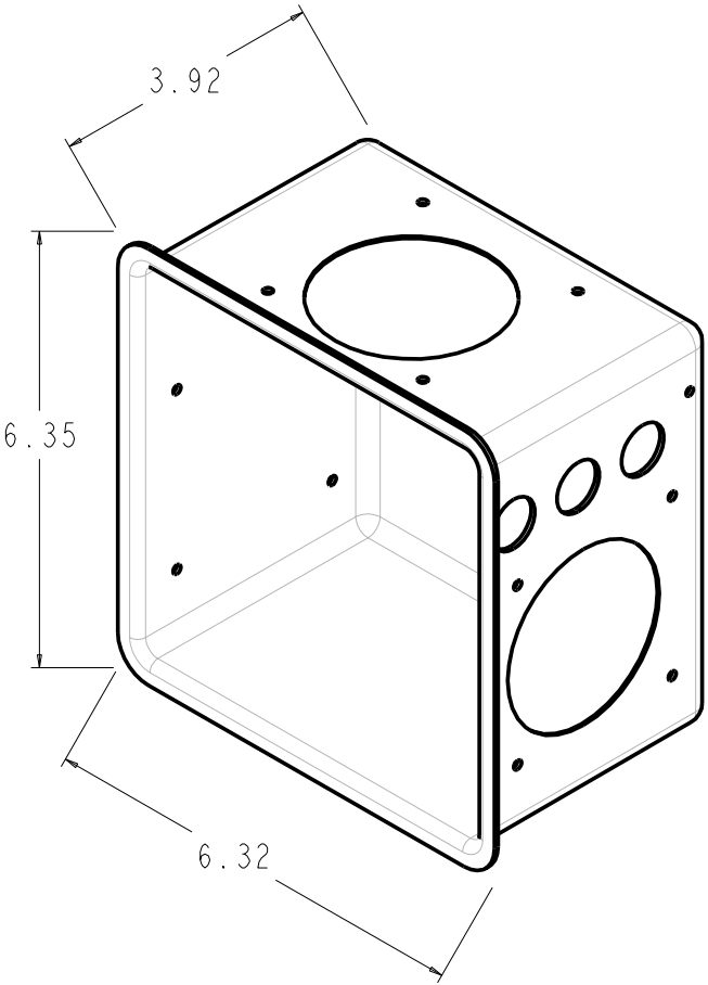
ELECTRICAL BOX
