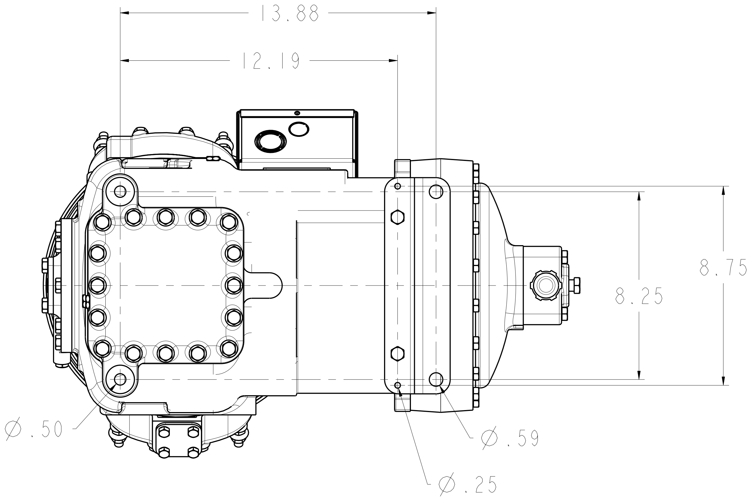
BOTTOM VIEW MOUNTING BOLT PATTERN
