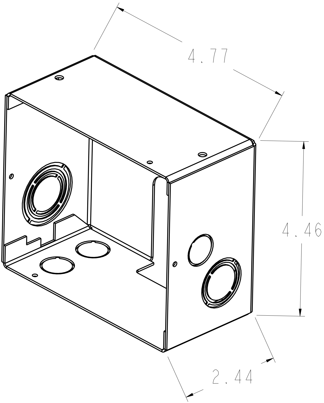
ELECTRICAL BOX KNOCKOUT SIZE COMBINATIONS
