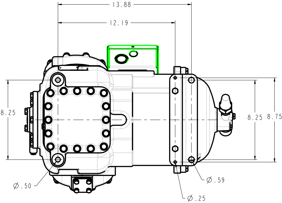
BOTTOM VIEW MOUNTING BOLT PATTERN
