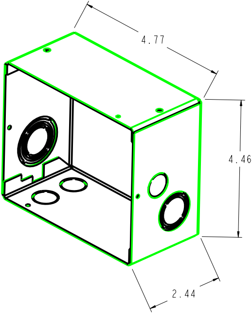
ELECTRICAL BOX KNOCKOUT SIZE COMBINATIONS
