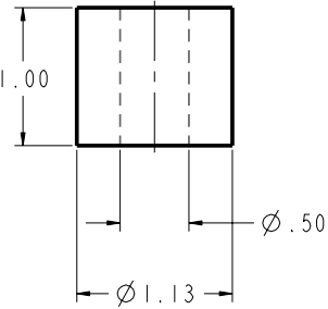
SCALE 2.000 30HR070-1071 SOLID MOUNT
