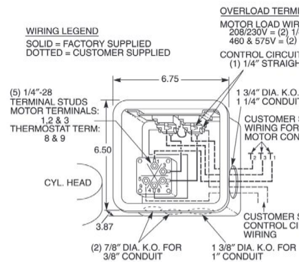
TERMINAL BOX DATA
