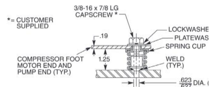
SPRING MOUNTING ARRANGEMENT
