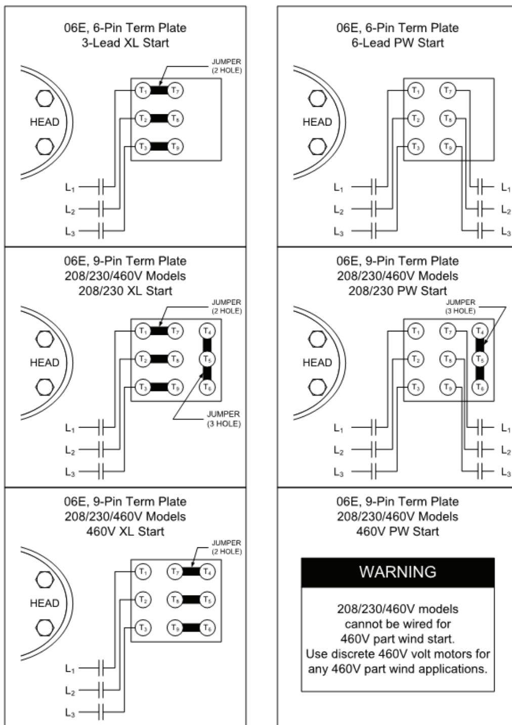
Fig. 16 — 06E Fixed Speed Wiring Diagrams
