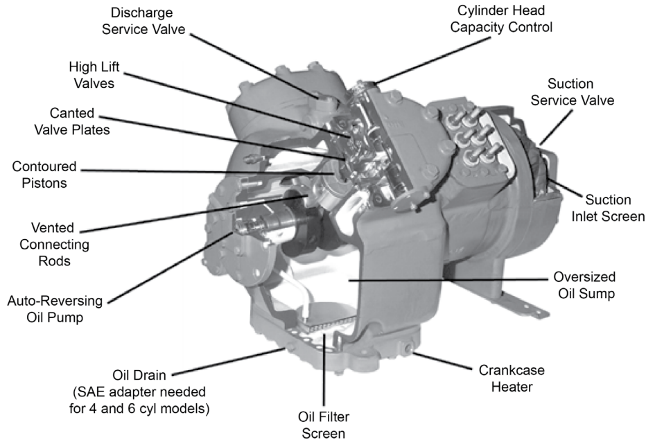
Fig. 1 — Key Features, 06E Semi-Hermetic Reciprocating Compressor
