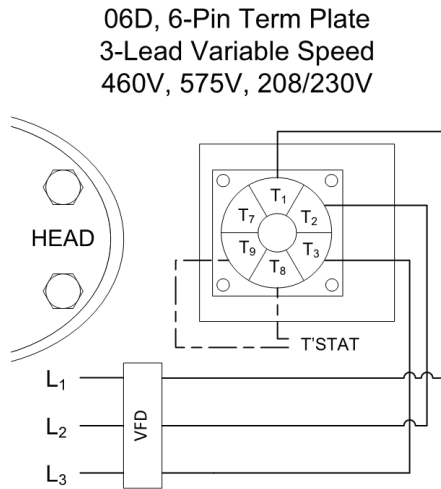
Fig. 15 — 06D Variable Speed Wiring Diagram
