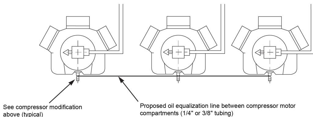
Fig. 12 — 06E Motor Barrel Equalization Line
