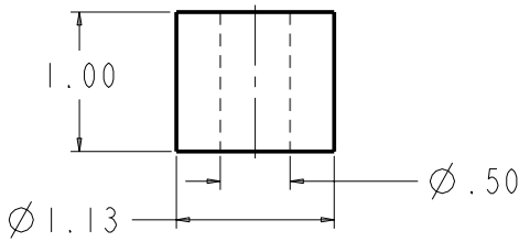
SCALE 2.000 30HR070-1071 SOLID MOUNT
