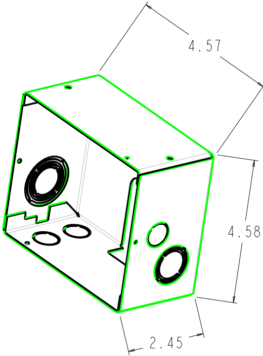
ELECTRICAL BOX KNOCKOUT SIZE COMBINATIONS
