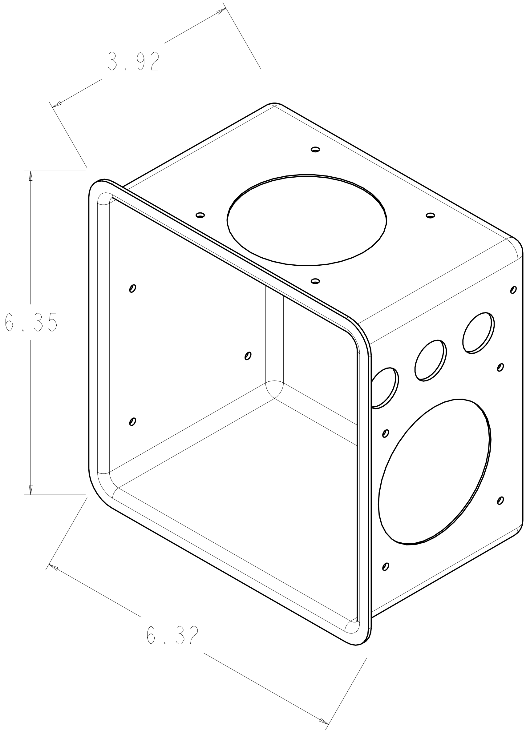
ELECTRICAL BOX
