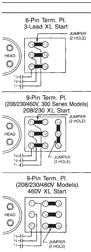
Fig. 30 — 06E Compressors (Across-the-Line [XL] Start)
