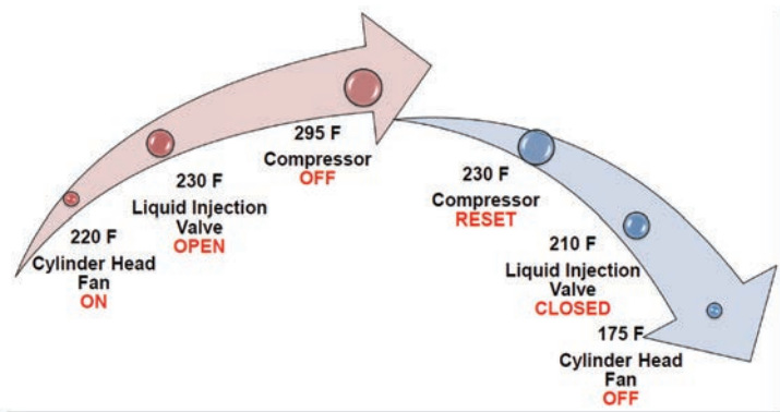
Fig. 39 — Discharge Temperatures
