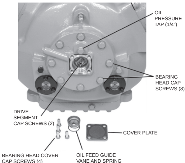
Fig. 8 — Removing Pump End Bearing Head (06E Compressor)
