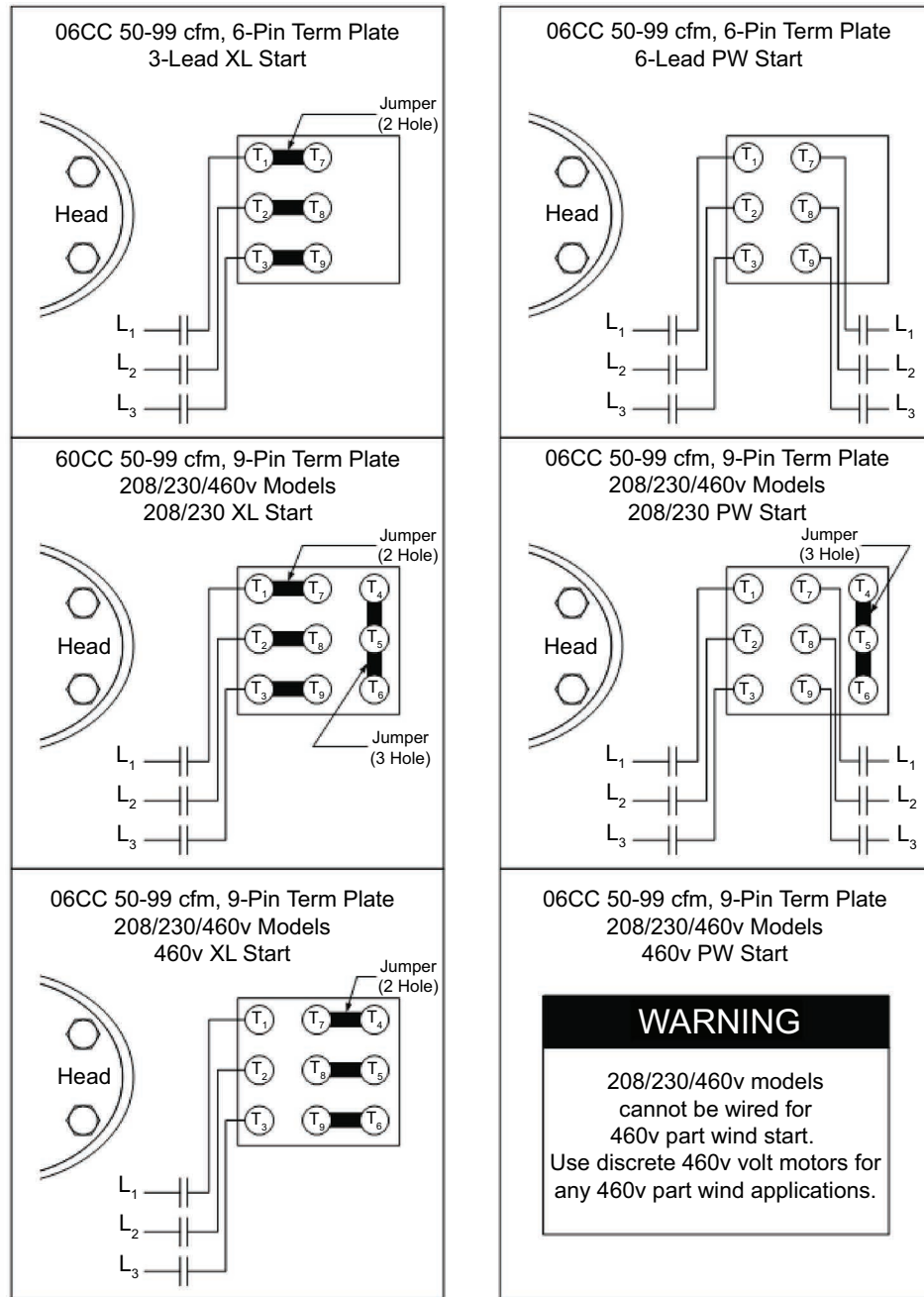
Fig. 15 — 06CC 50-99 cfm Fixed Speed Wiring Diagrams
