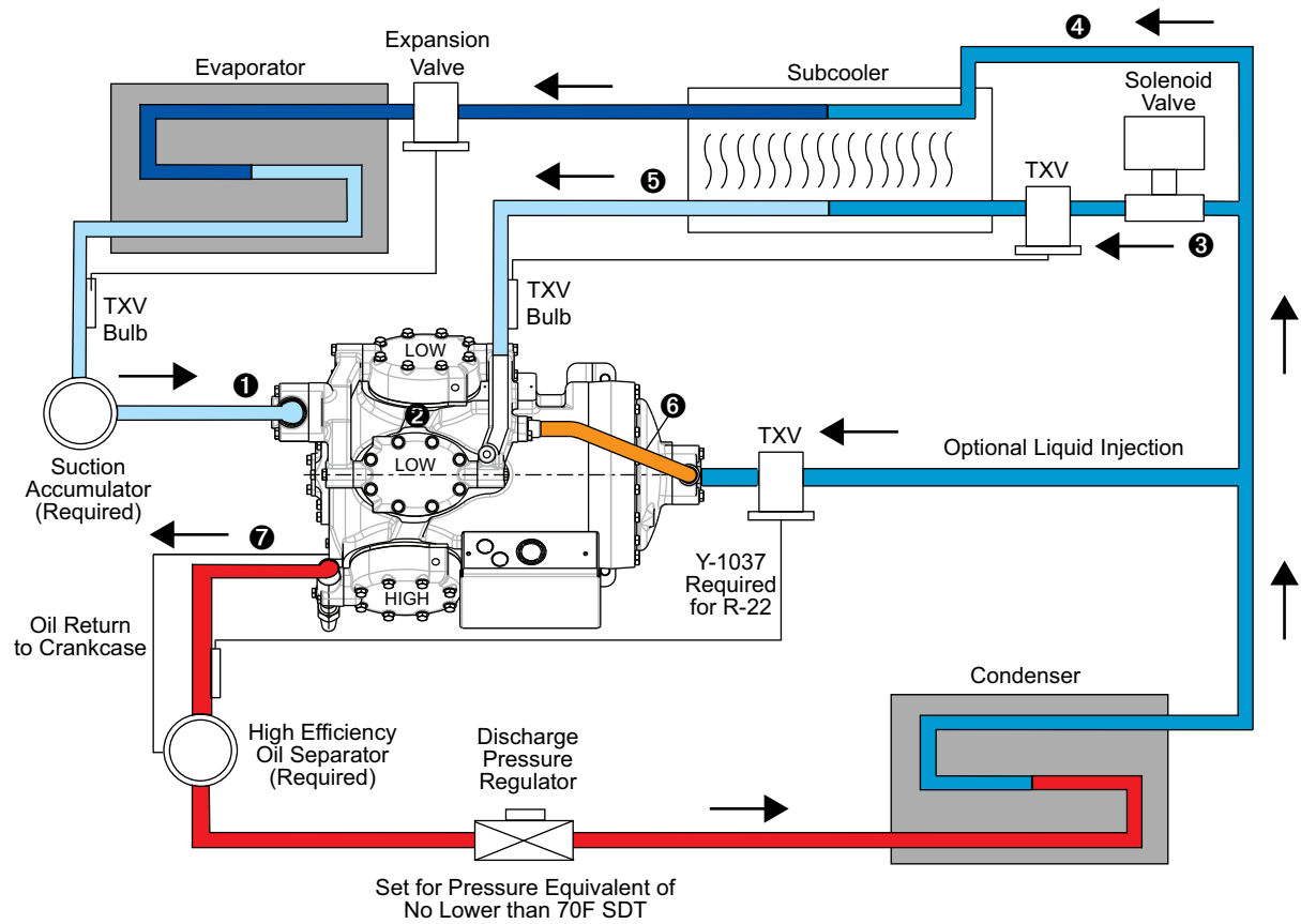
Fig. 8 — Single Compressor 06CC System Piping
