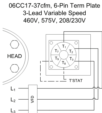
Fig. 14 — 06CC 17-37 cfm Variable Speed Wiring Diagram
