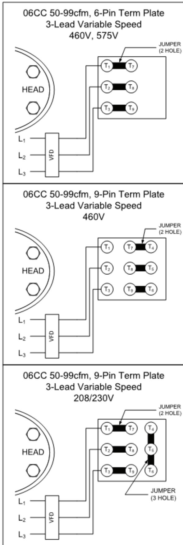
Fig. 17 — 06CC 50-99 cfm Variable Speed Wiring Diagrams
