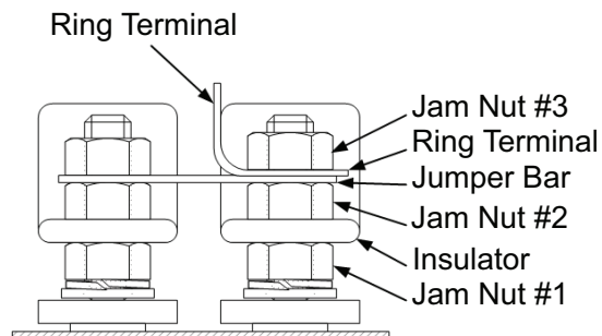
06CC 50-99 cfm Terminal Pin Wiring Detailed View
