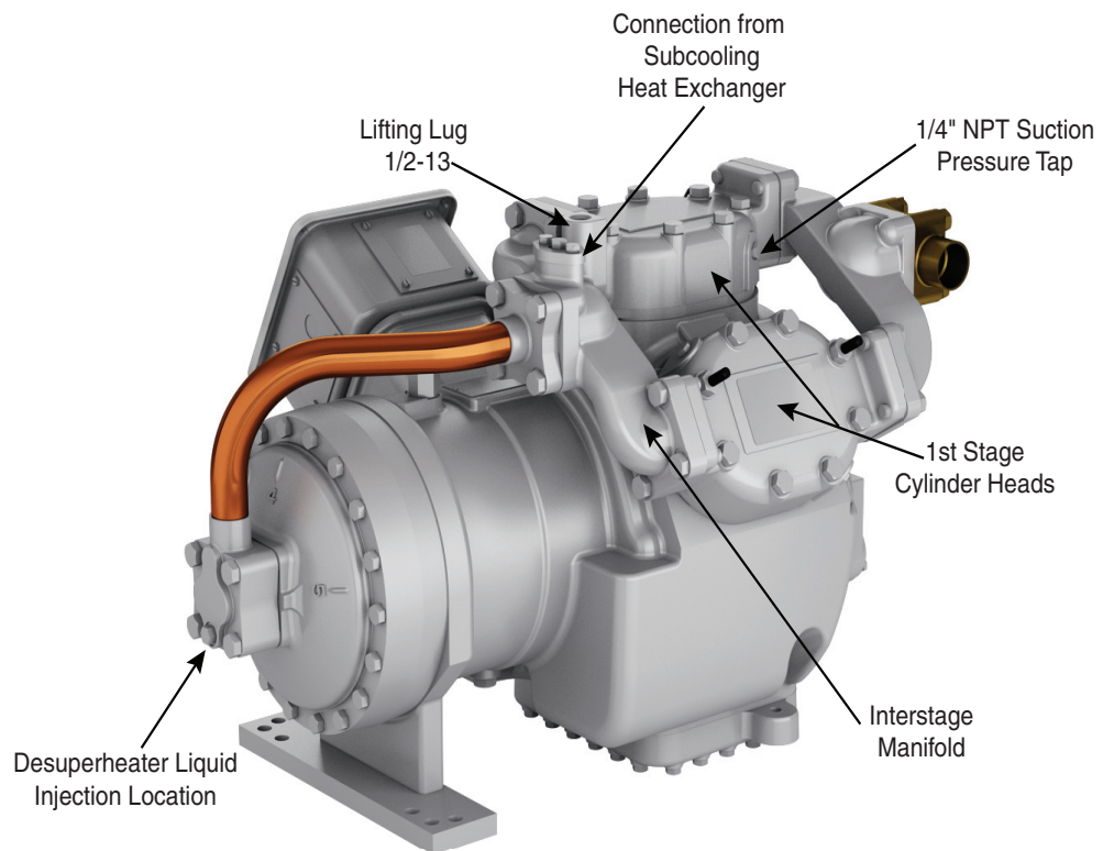
Fig. 3 — Key Features, 06CC 50-99 cfm Compressor Models
