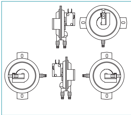
Fig. 1: Mount with the diaphragm in any vertical plane. Sample line connections must not point upward.
