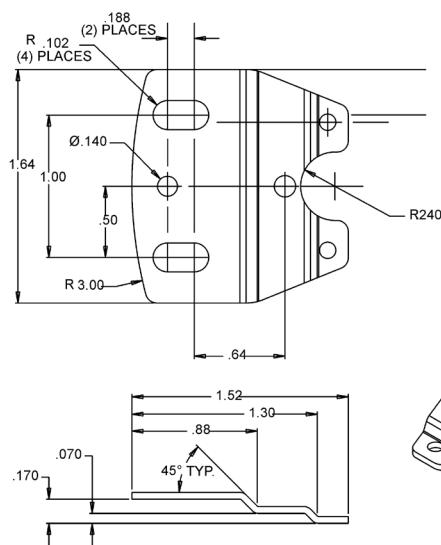
Figure 5: "L" Bracket
