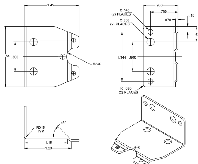
Figure 5: "L" Bracket
