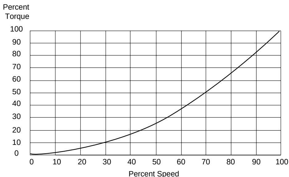
Figure 9 Variable Torque Loads
