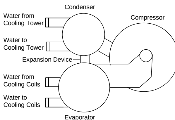
Figure 7 Chiller
