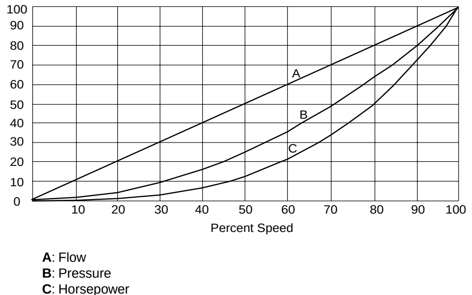
Figure 10 The Affinity Laws
