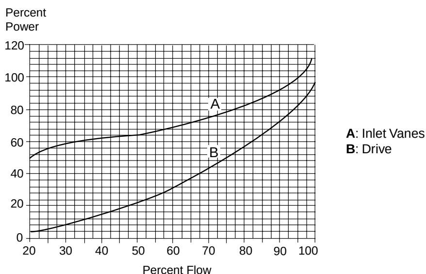
Figure 13 Fan Performance
