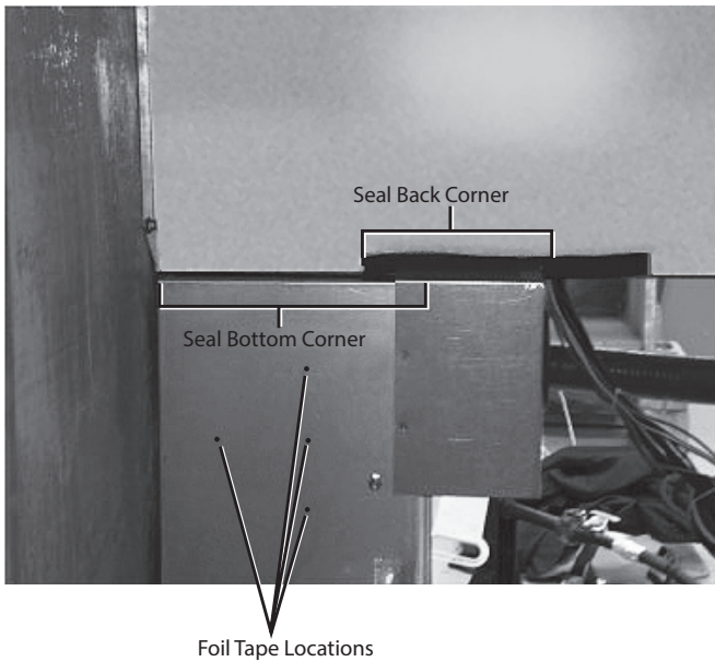
Fig. 29 — Seal Strip and Foil Tape Locations
