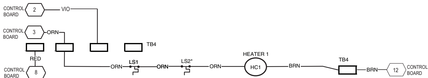
Fig. 41 — Electric Heater Control Connections - Air Conditioner with CRHEATER288A00-293A00
