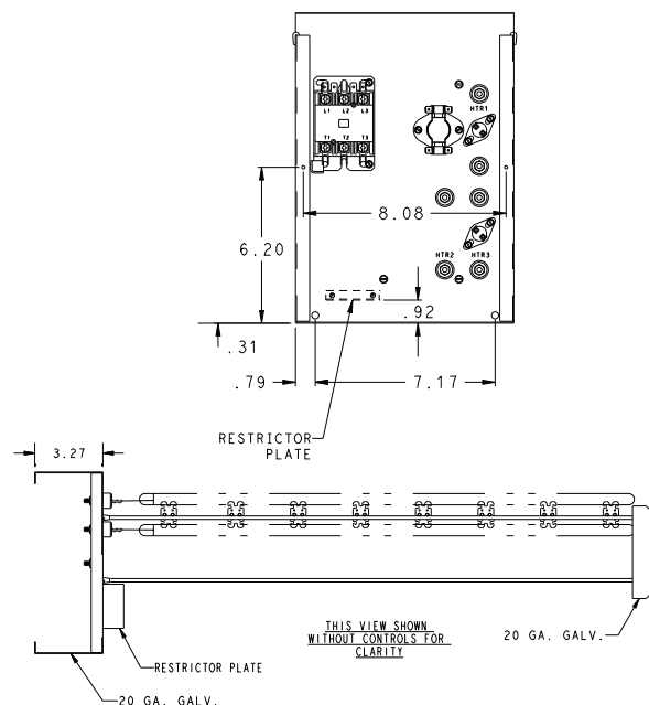
Fig. 35 — Restrictor Plate
