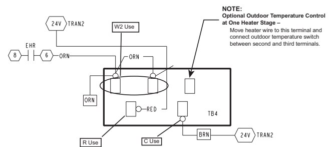
Fig. 39 — TB4 Terminal Use (HP Only)
