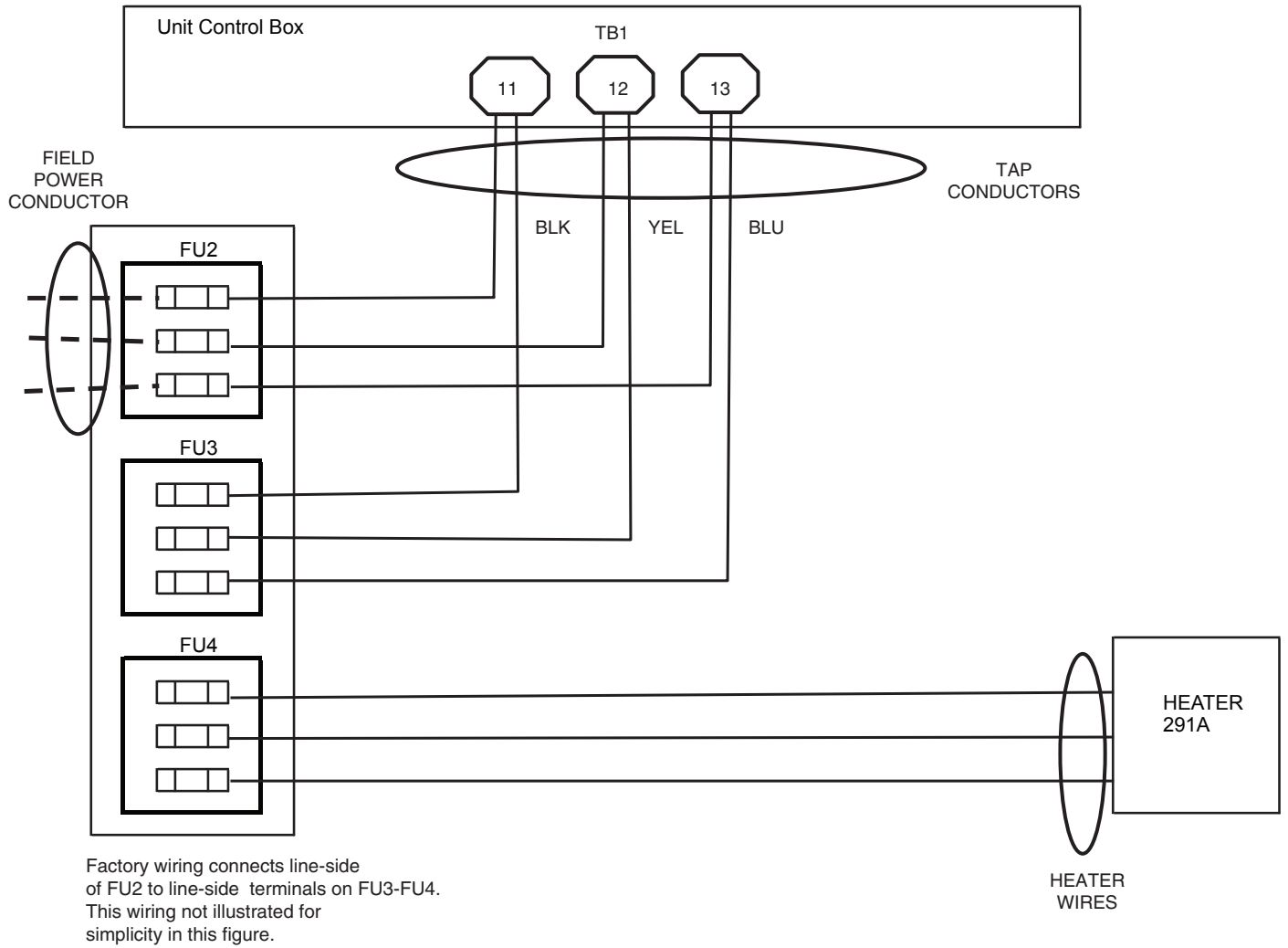
Fig. AO — Heat Pump Single Point Box CRSINGLE051A00 (HP-1, Size 14)
