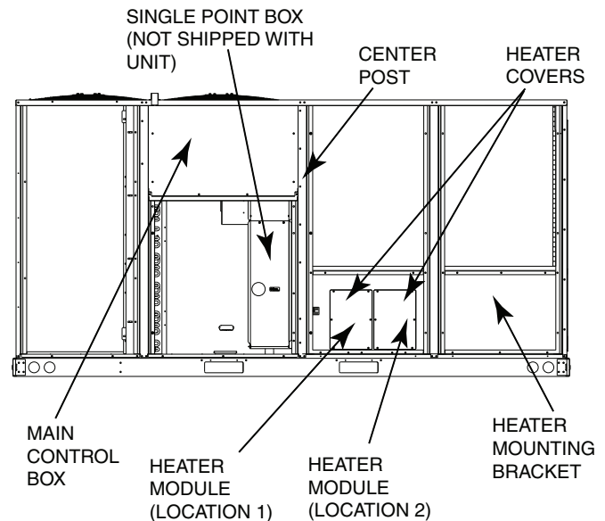
Fig. 26 — Typical Component Location
