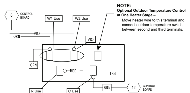
Fig. 40 — TB4 Terminal Use (AC Only)
