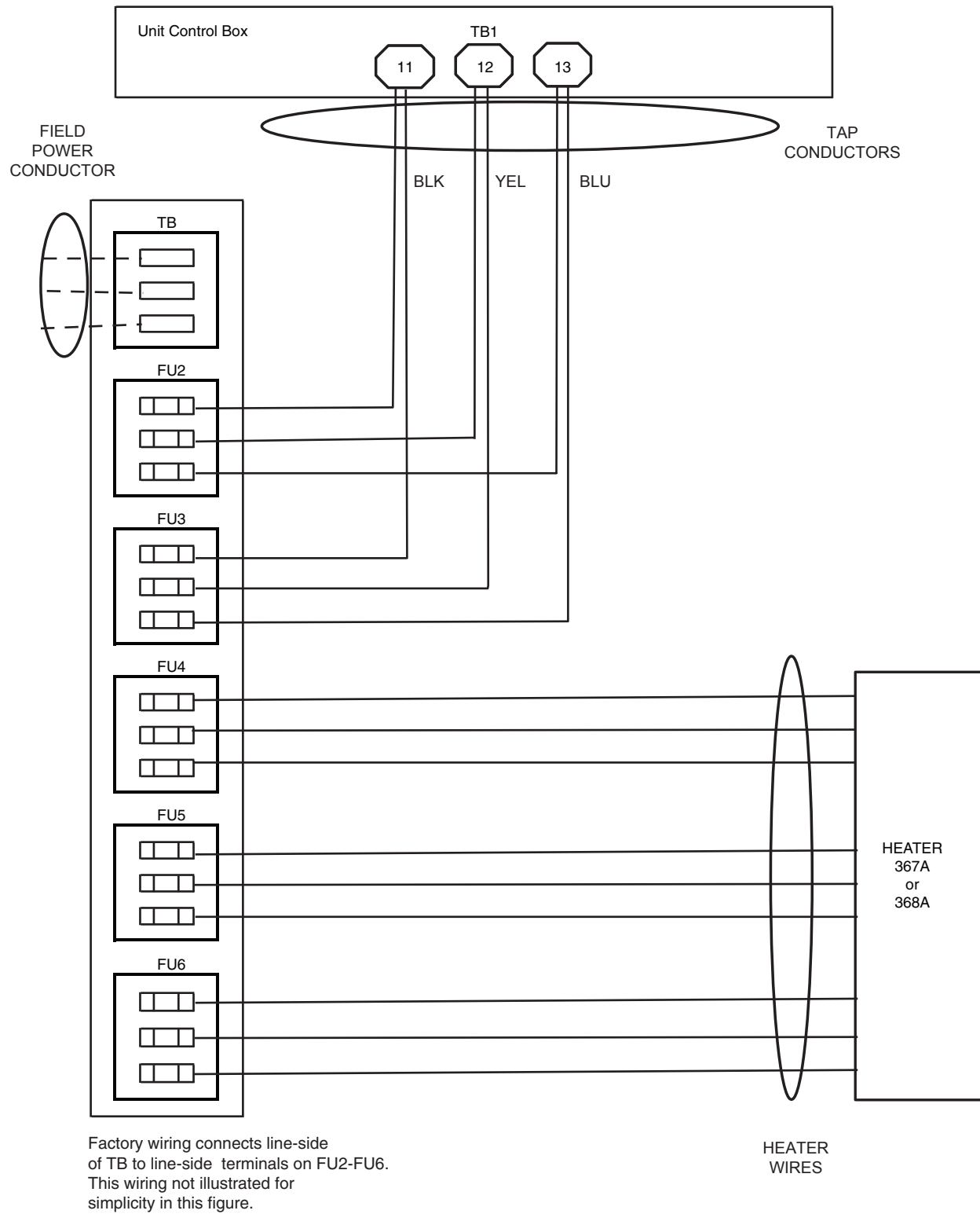
Fig. T — AC Single Point Box CRSINGLE054A00 (AC-2, Size 14)
