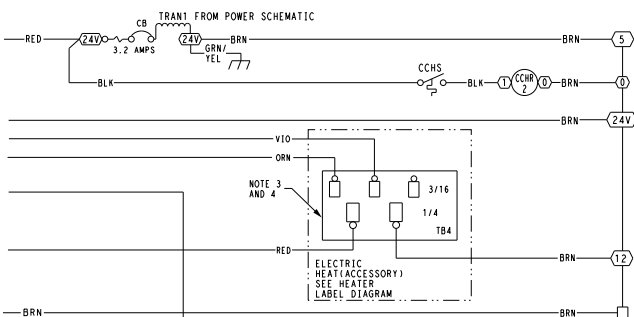
Fig. 38 — TB4 Wiring (AC Only)
