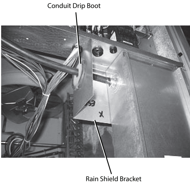
Fig. 30 — Rain Shield Installation
