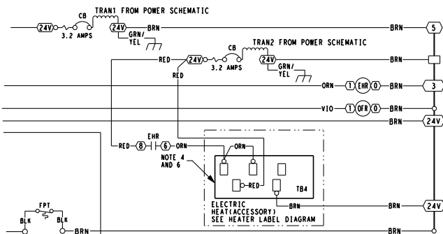
Fig. 37 — TB4 Wiring (HP Only)
