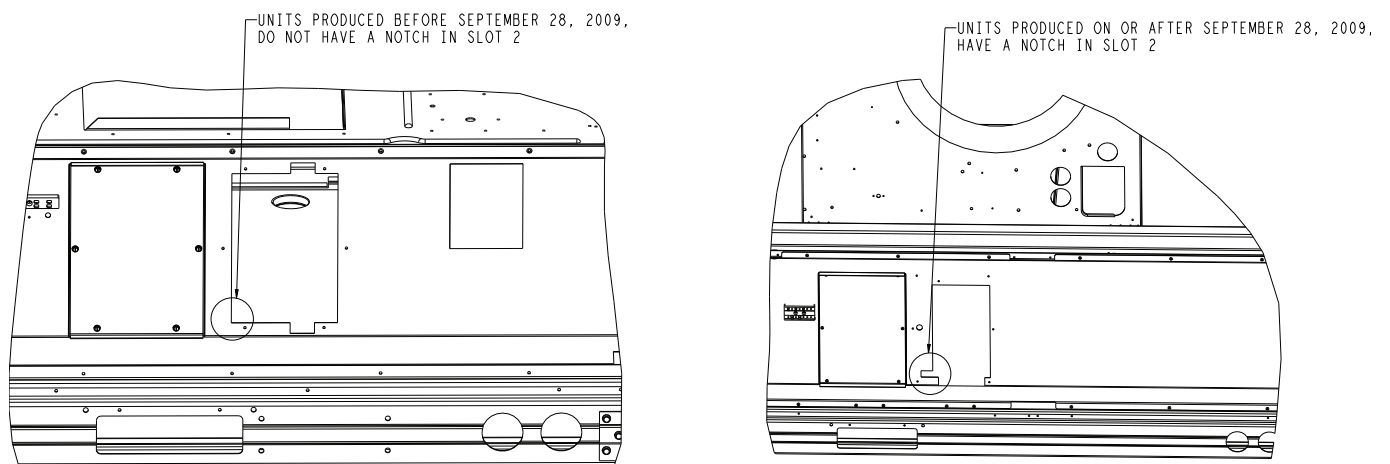
Fig. 12 — Slot 2 with and without Notch
