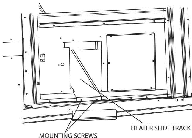
Fig. 34 — Heater Slide Track Installation
