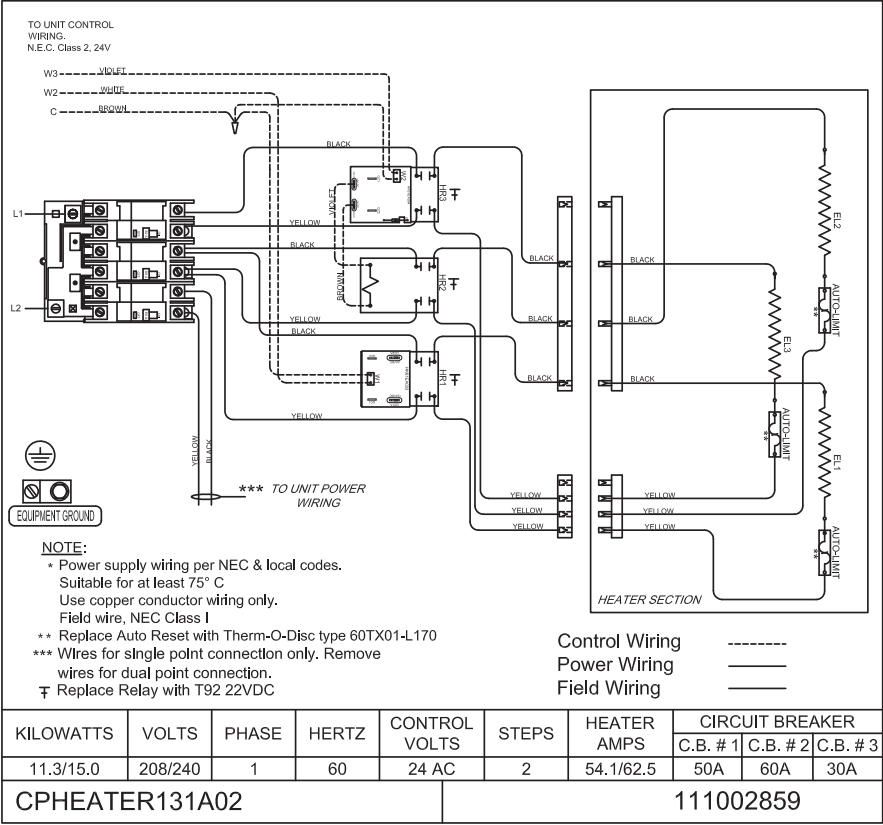
Fig. 20 - CPHEATER131A02 Wiring Diagram
