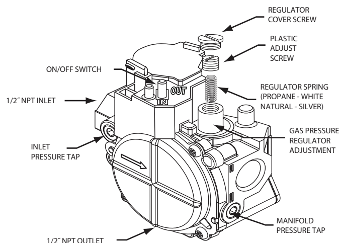
Single-Stage 36G Valve
