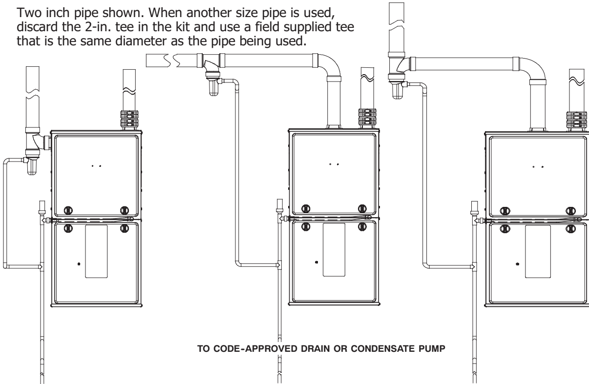
Fig. 11 – Application of Trap Kit to Combustion Air Pipe Located Above Furnace
