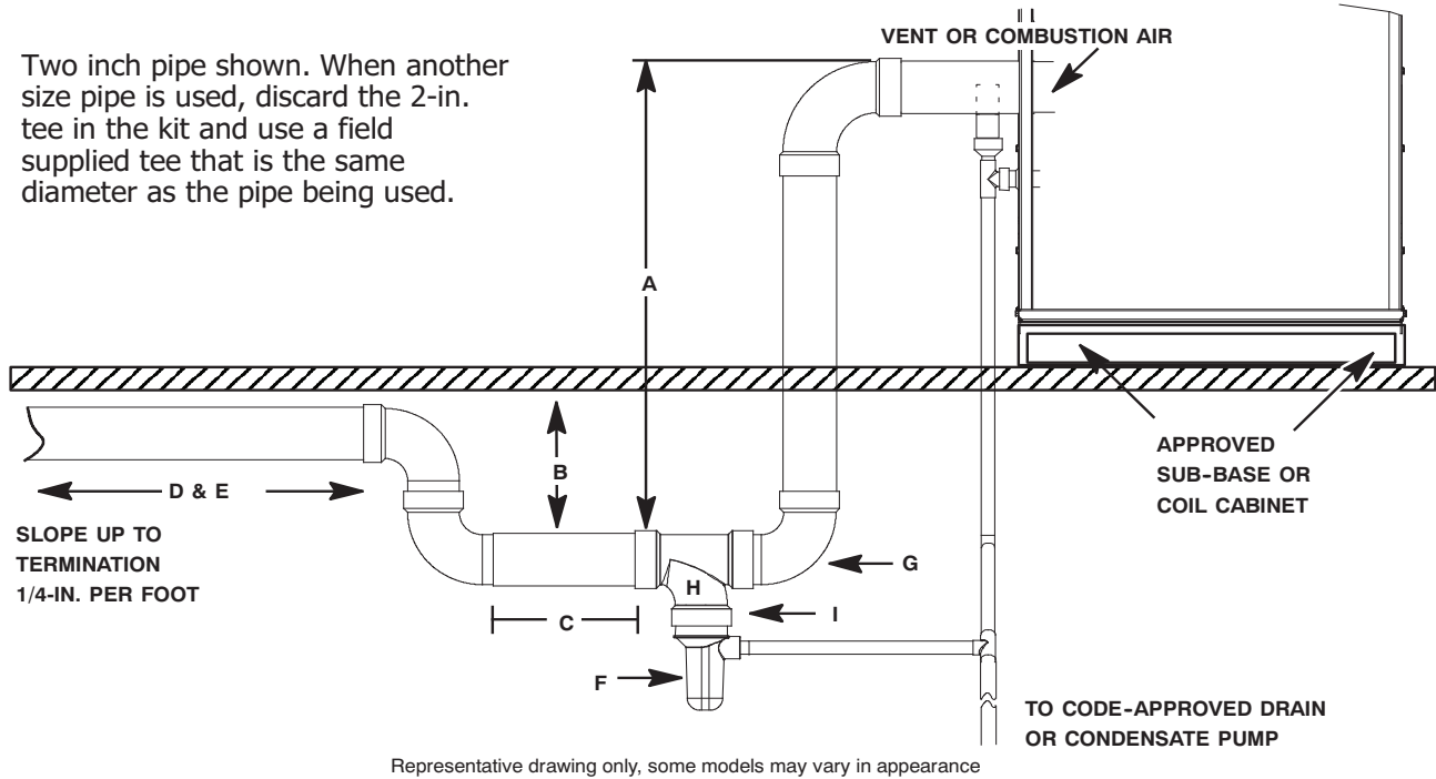
Fig. 1 – Condensate Trap Plumbing Options for Vent or Combustion Air Pipe Below Furnace
