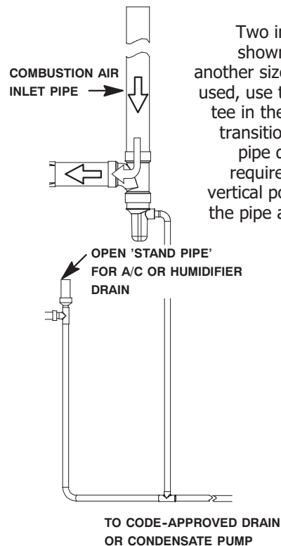
Fig. 3 – Condensate Trap Plumbing Options for Combustion Air Pipe (ONLY) Above Furnace
