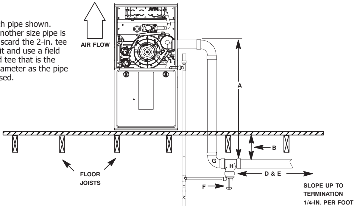
CONFIGURATION FOR VENT AND/OR COMBUSTION AIR PIPING (See NOTES in Figure 1)
