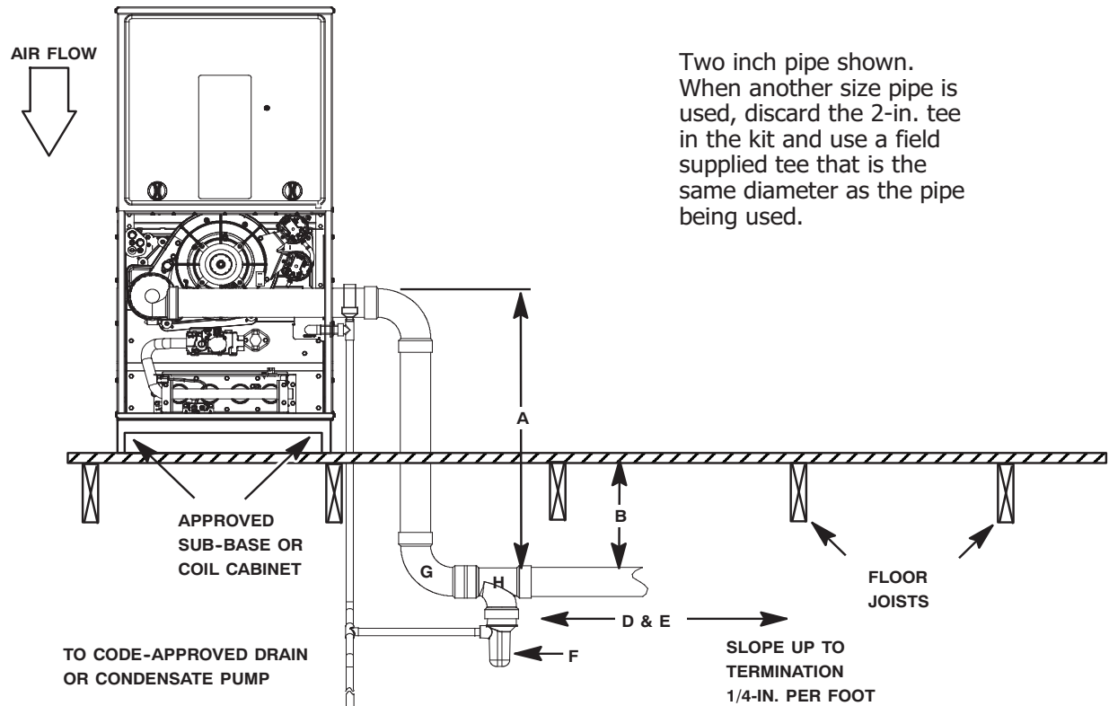
CONFIGURATION FOR VENT AND/OR COMBUSTION AIR PIPING (See NOTES in Figure 1)
