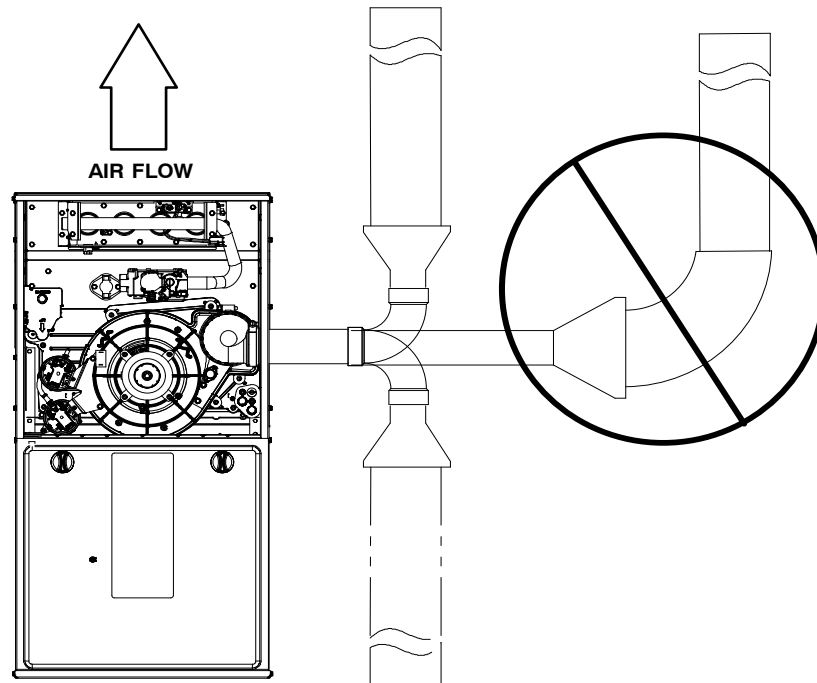
Fig. 11 – Application of Trap Kit to Combustion Air Pipe Located Above Furnace
