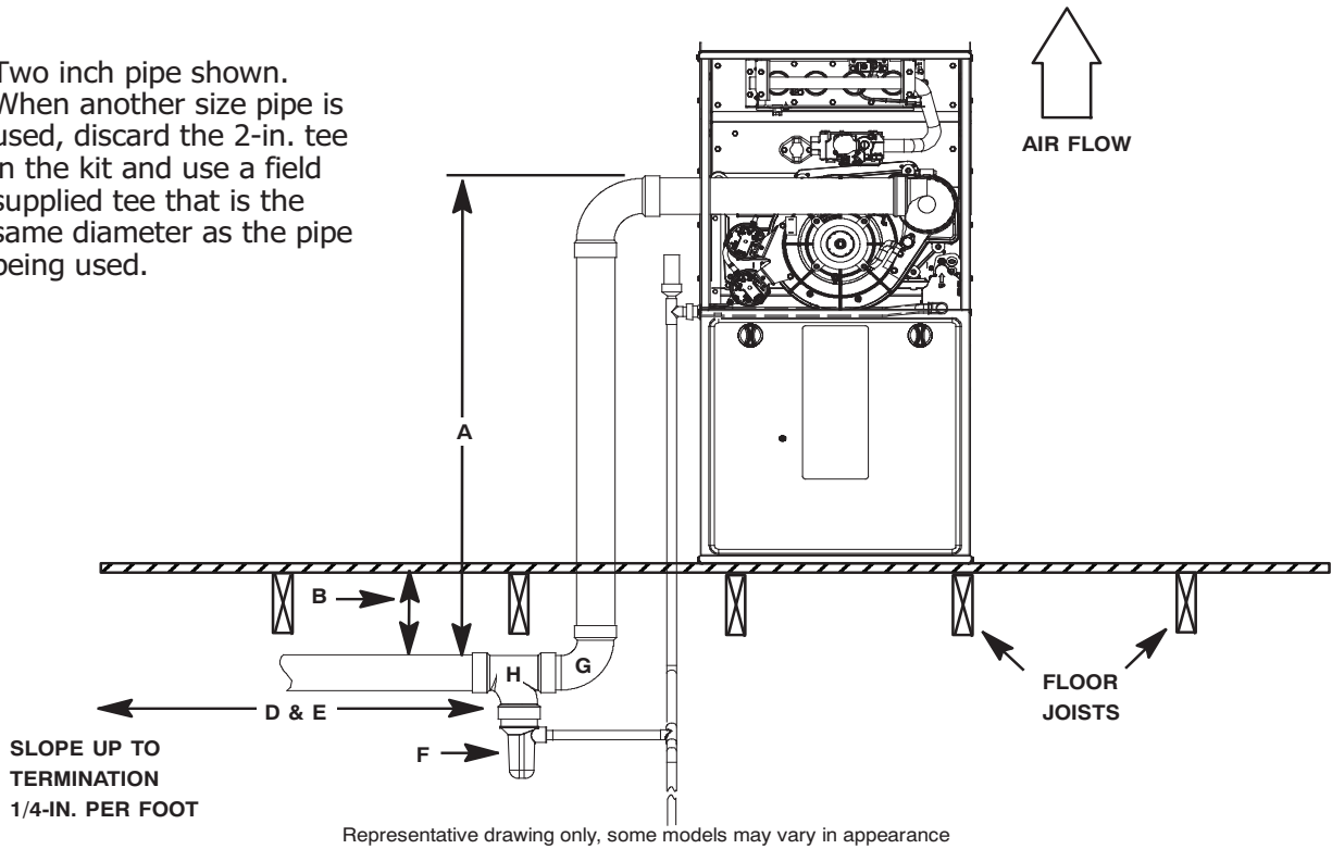
Fig. 5 – Vent Located Below Floor with Upflow Furnace and Side Venting
