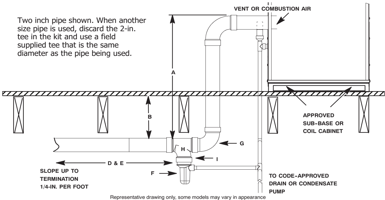
Fig. 2 – Condensate Trap Plumbing Options for Vent or Combustion Air Pipe Below Furnace
