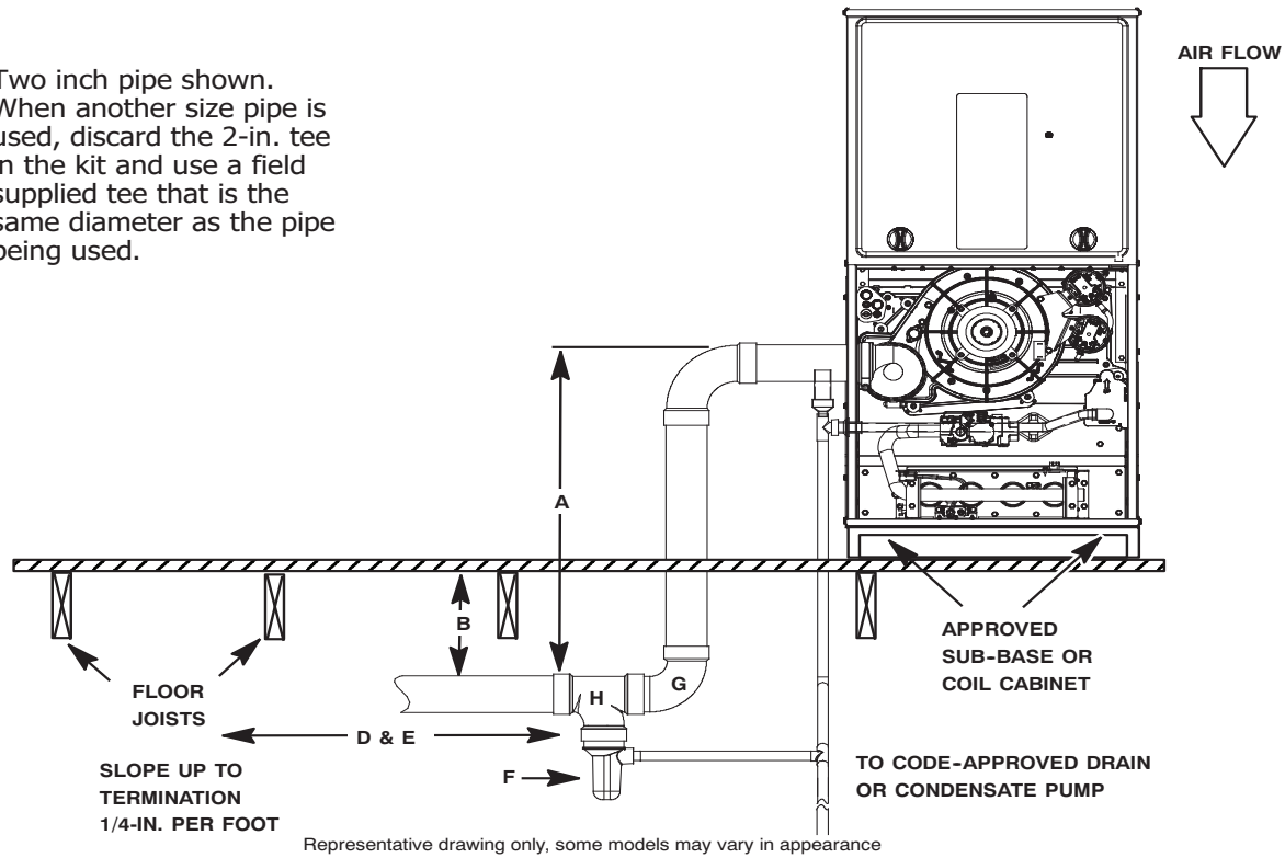
Fig. 7 – Vent Located Below Floor with Downflow Furnace and Side Venting
