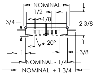
LTM 1/2 20°
