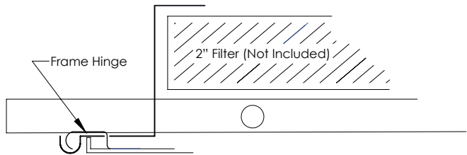
105PTFG Frame Detail
