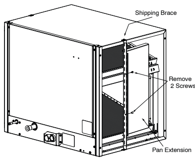
Fig. 1 - Furnace Coil
