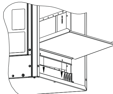
Fig. 3 - Horizontal-Right Installation of Pan Extension (43, 60, & 61 sizes only)
