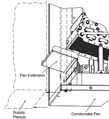
Fig. 2 - Horizontal-Left Installation of Pan Extension (43, 60 & 61 sizes only)
