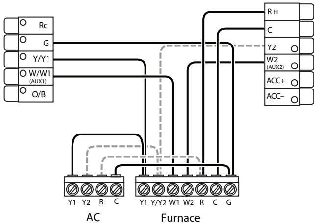
Fig. 10 - Air Conditioner- Two Stages each (Heat / Cool)
