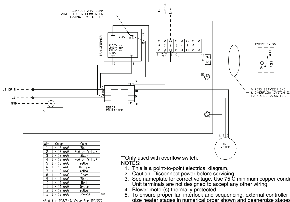
Fig. 99 — 42B Motor Controls — Single-Phase Only
