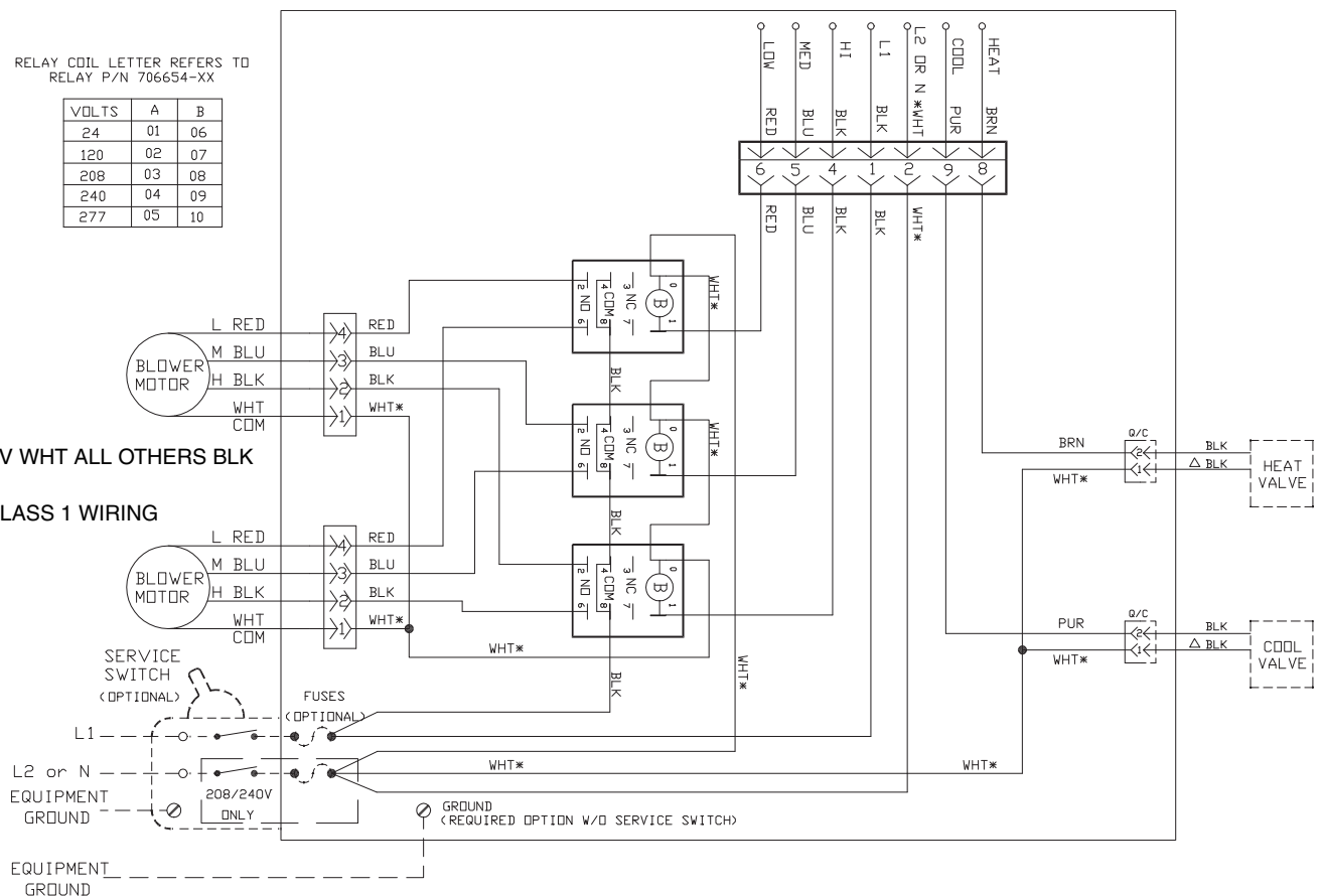
Fig. 77 — 42C,S,V (except VG) and 42D (600-1000 cfm) 4-Pipe Heating and Cooling — Line Voltage Control by Others
