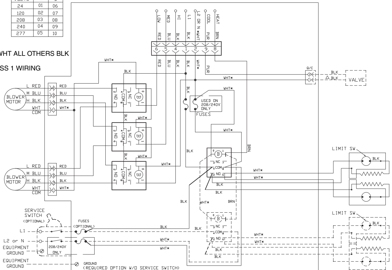
Fig. 61 — 42D (1200-2000) 2-Pipe Cooling with Total Electric Heat — Field-Supplied and Installed Controls (Line Voltage and Control Valves or Electric Heat)
