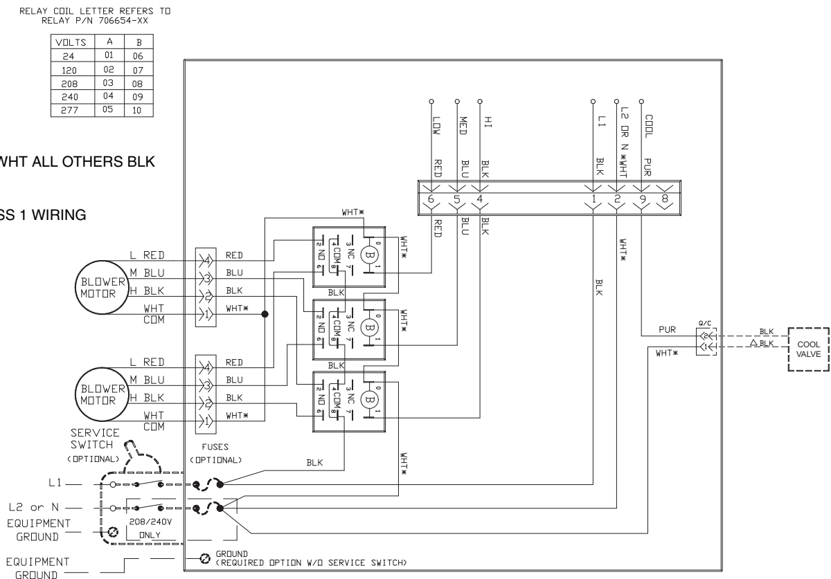
Fig. 4 — 42D (1200-2000) 2-Pipe Cooling Only — Field-Supplied and Installed Controls (Line Voltage and Control Valves)
