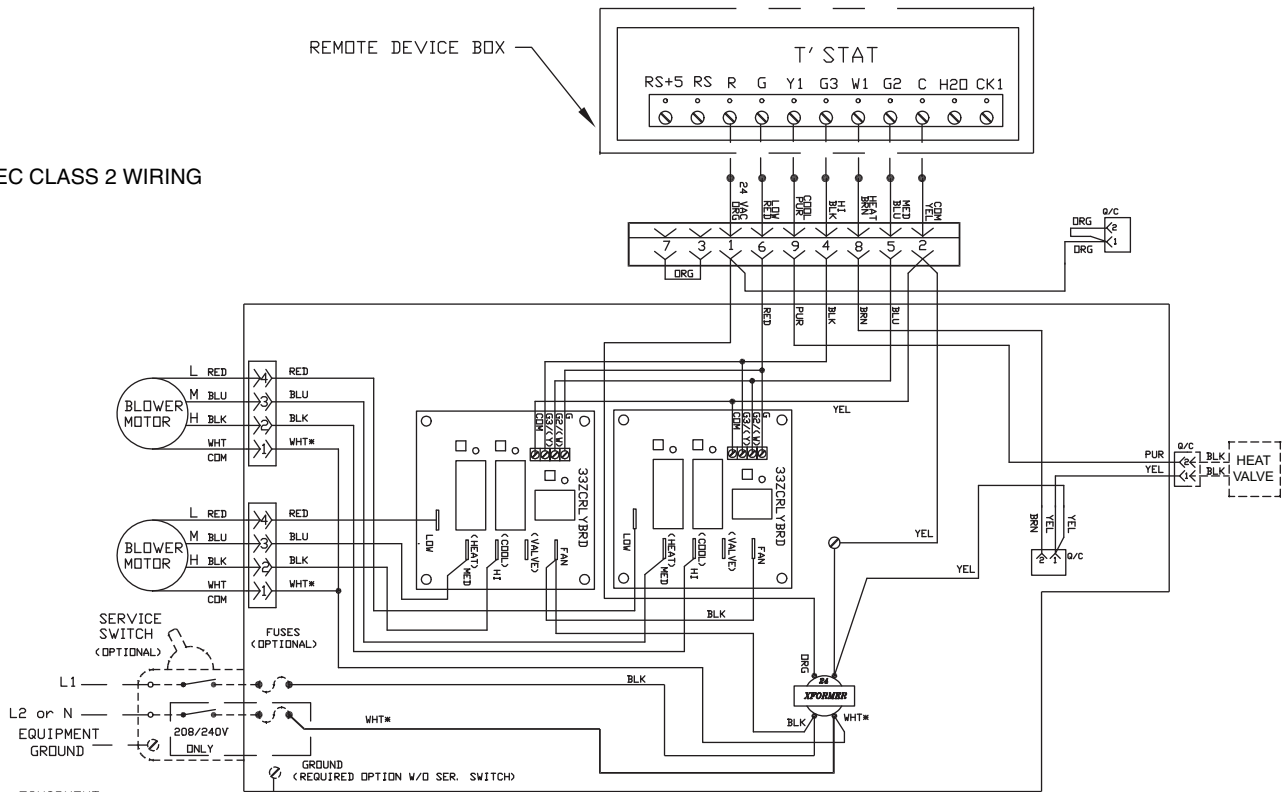
Fig. 21 — 42D (1200-2000) 2-Pipe Heating Only — Remote/Wall-Mounted Debonair Thermostat (24-v)
