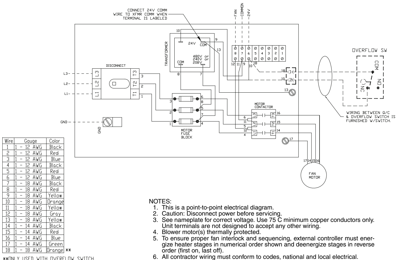
Fig. 102 — 42B Motor Controls — 3-Phase with Interlocking Disconnect
