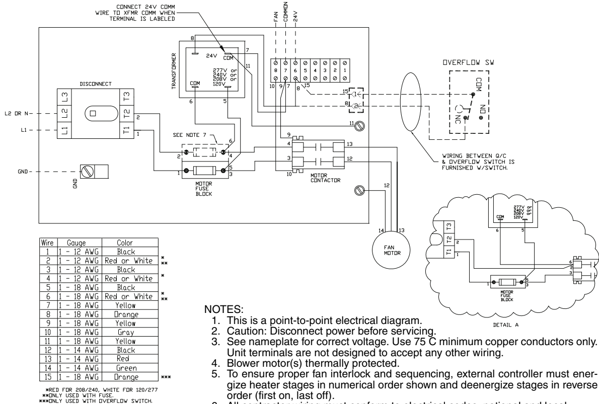
Fig. 100 — 42B Motor Controls — 3-Phase Only
