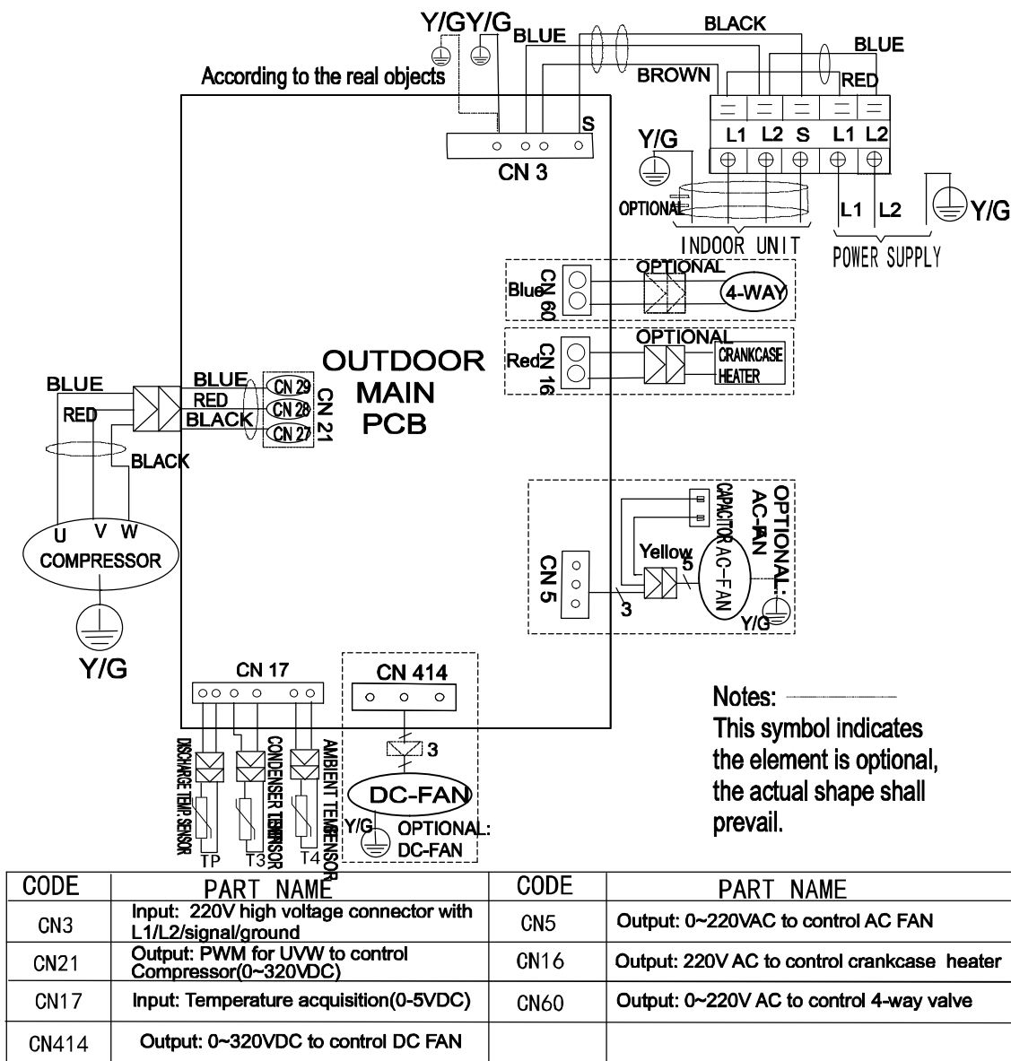
Fig. 8 – Wiring Diagram Cooling Only Sizes 18–24K
