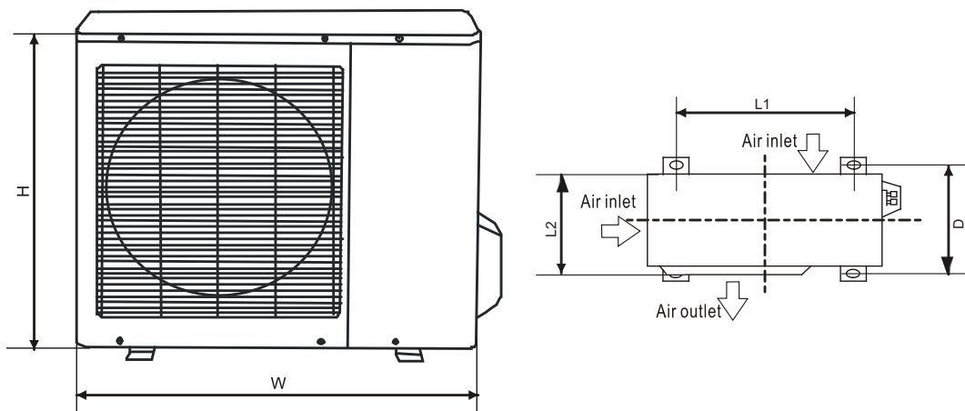
Fig. 3 – Dimensions – Outdoor
