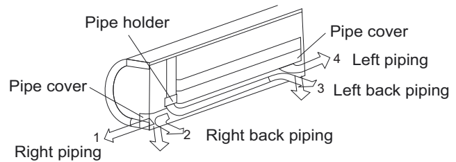
Fig. 7 – Piping Locations
