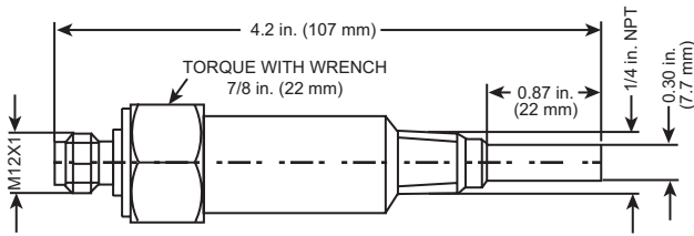
Fig. 27 — Thermal Flow Sensor
