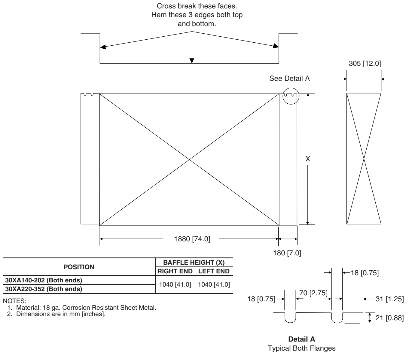
Fig. 29 —Field-Fabricated and Field-Installed Wind Baffles
