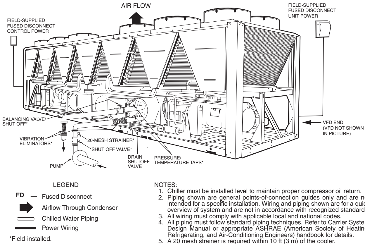
Fig. 18 — 30XA Flooded Cooler Typical Piping and Wiring
