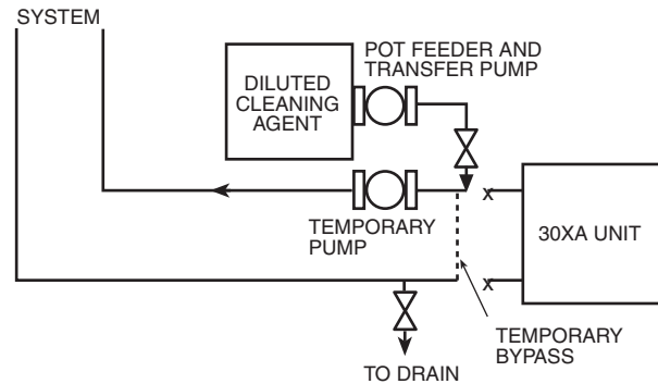
Fig. 30 — Typical Set Up for Cleaning Process
