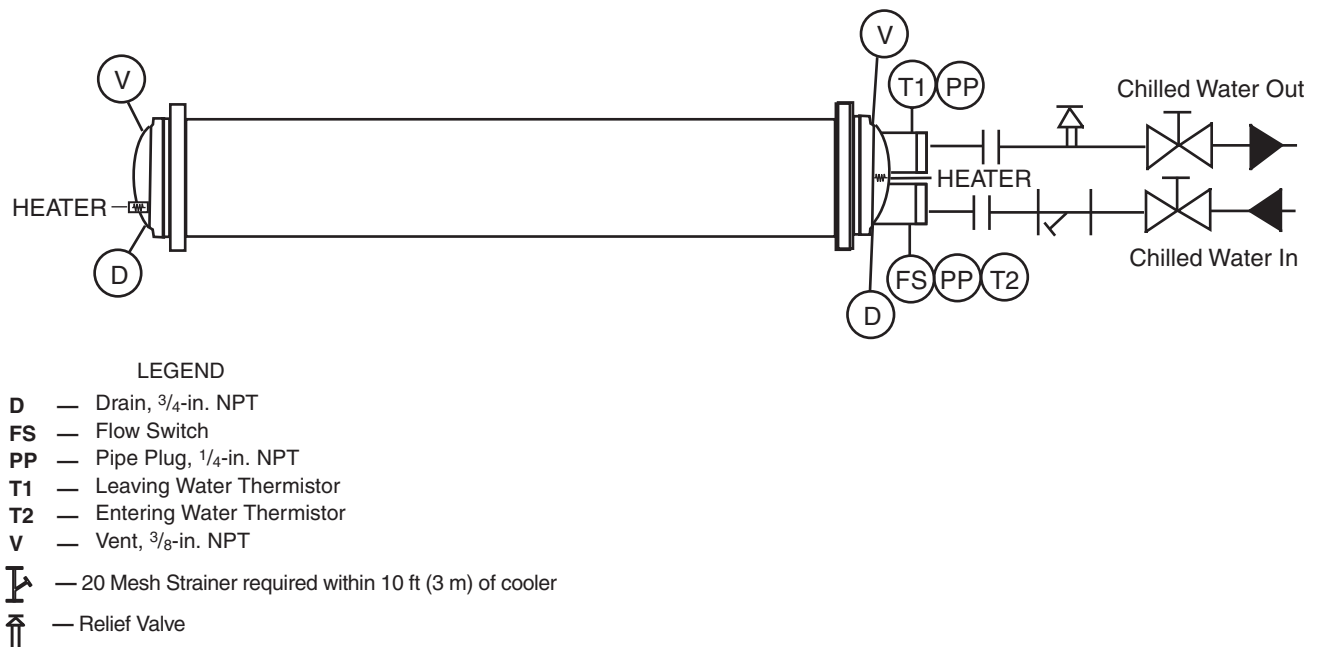
Fig. 24 — Typical Piping Diagram for 30XA Units with Greenspeed® Intelligence
