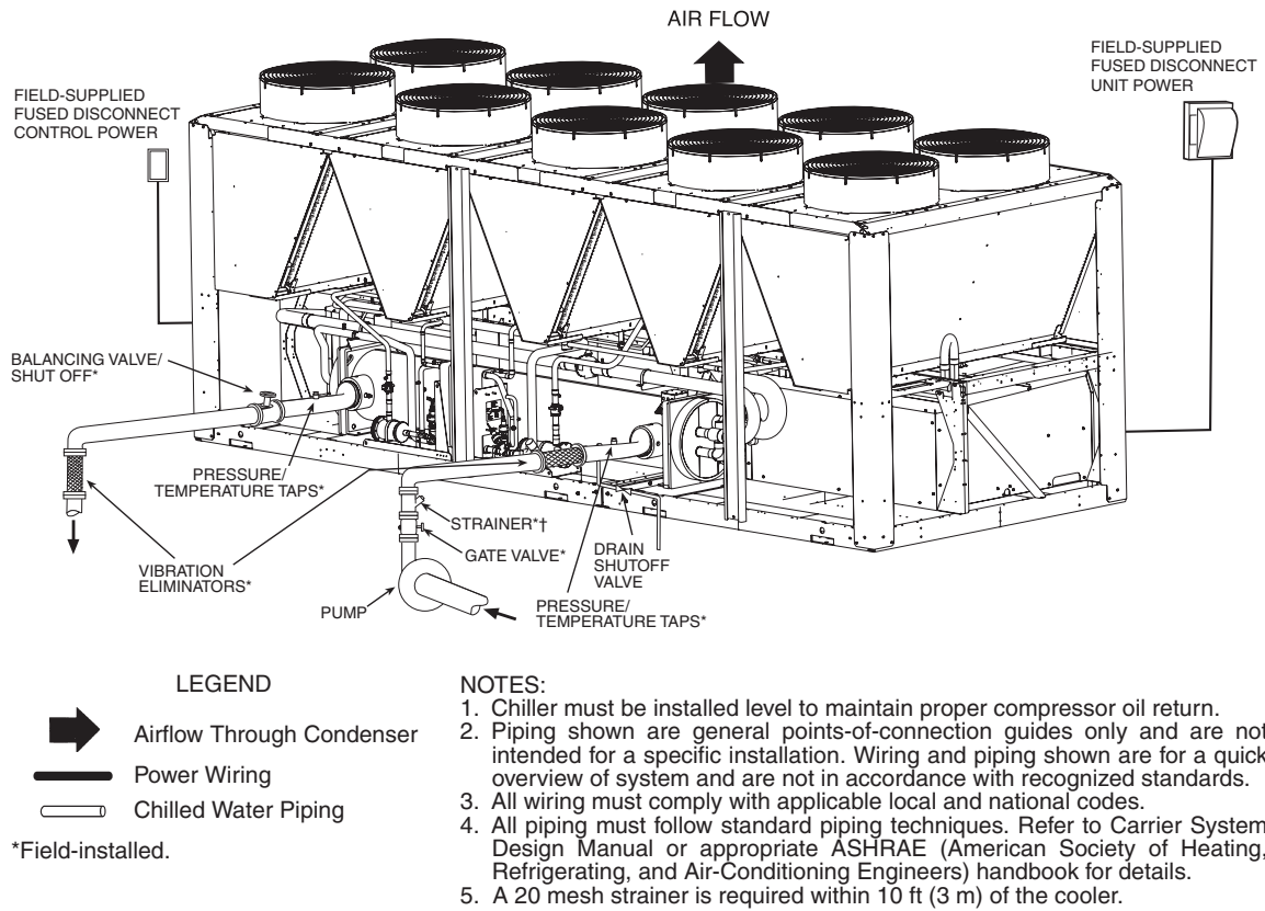
Fig. 19 — 30XA DX Cooler Typical Piping and Wiring
