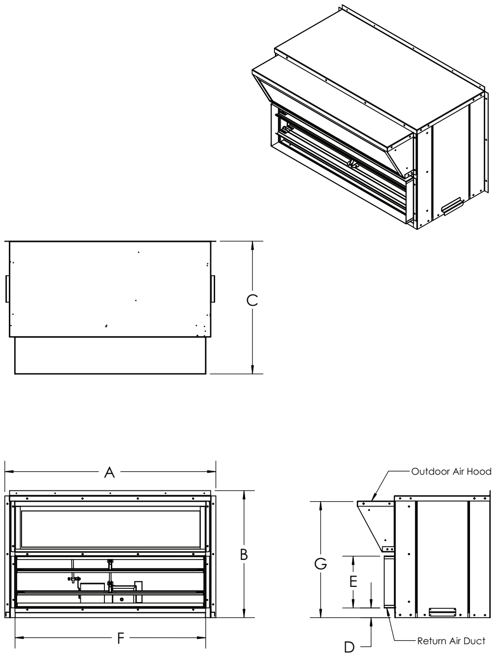
DIMENSIONS (in.)
