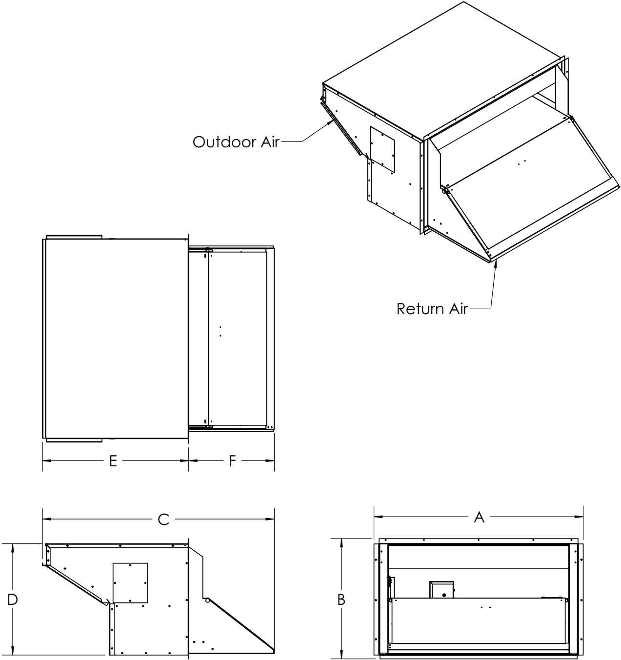
DIMENSIONS (in.)
