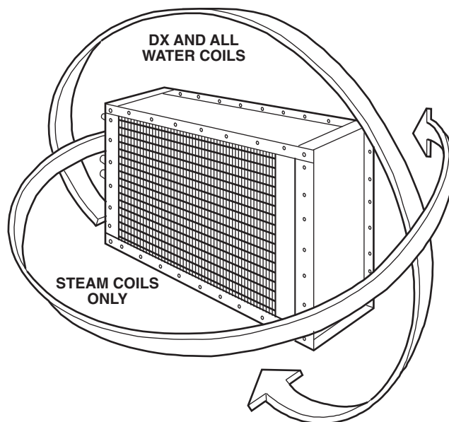
Fig. 176 — Coil Rotation
