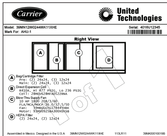
Fig. 1 — 39MN Unit Nameplate Label
