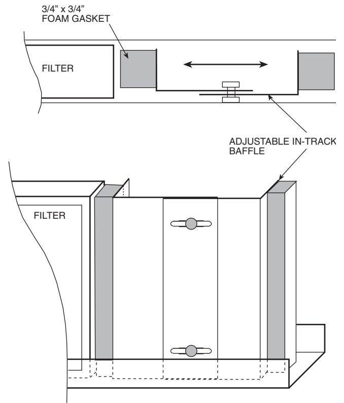
Fig. 182 — In-Track Baffle for Flat, Angle and Sideload Bag/Cartridge Filter Sections
