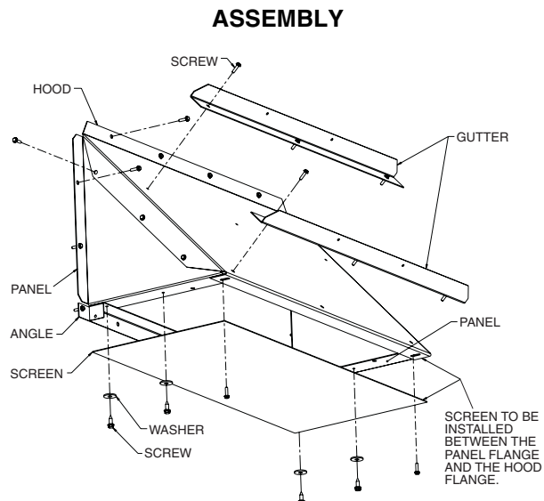
Fig. 51 — Collapsible Exhaust Box Hood
