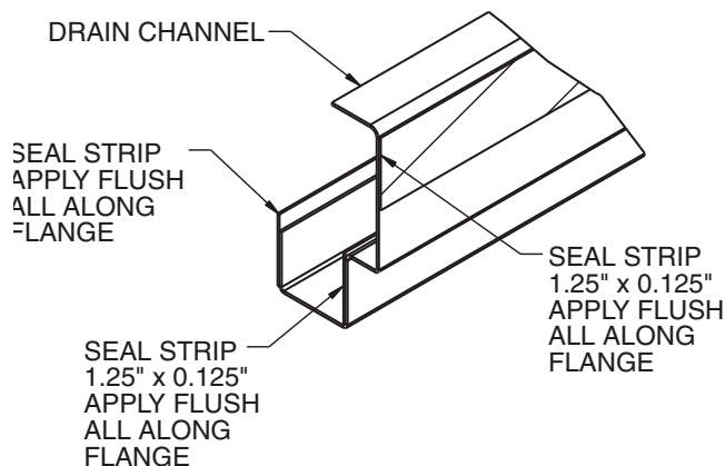
Fig. 57 — Applying Seal Strip to Roof Drain Channel
