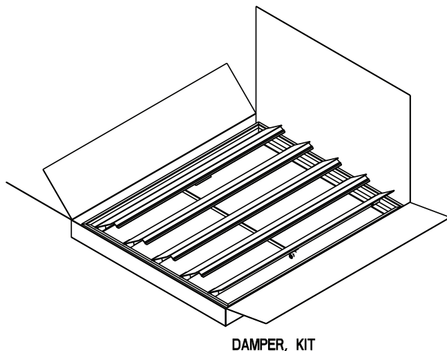
Fig. 67 — Power Exhaust Damper Kit
