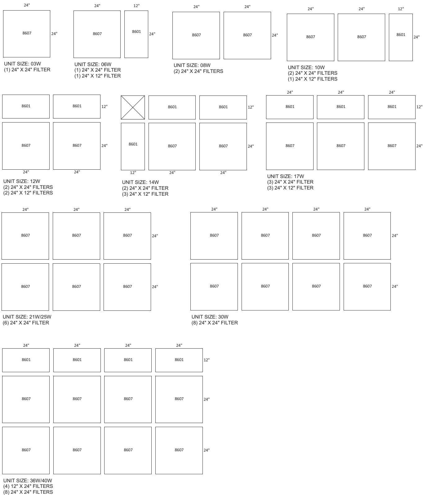
Fig. 188 — Front Load Bag/Cartridge Filter Arrangement
