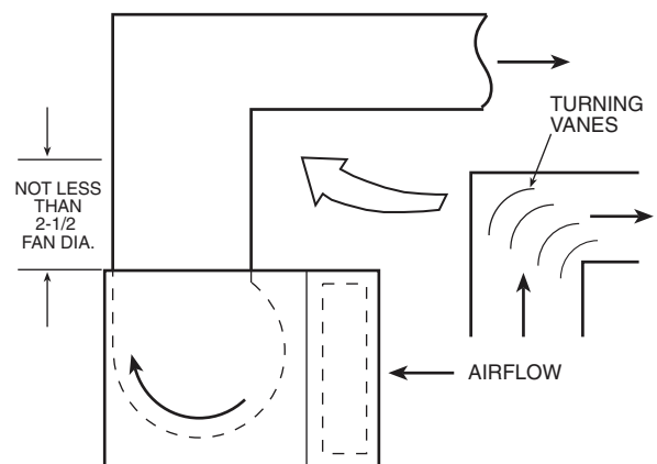
Fig. 33 — Recommended Discharge Duct Arrangement When Turns are Required
