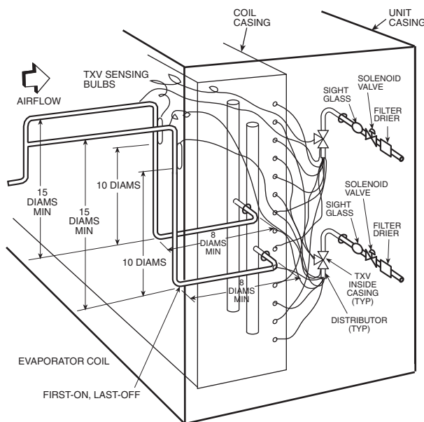
Fig. 96 — Row Split Coil Suction-Line Piping
