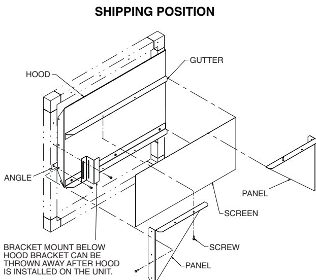
Fig. 51 — Collapsible Exhaust Box Hood
