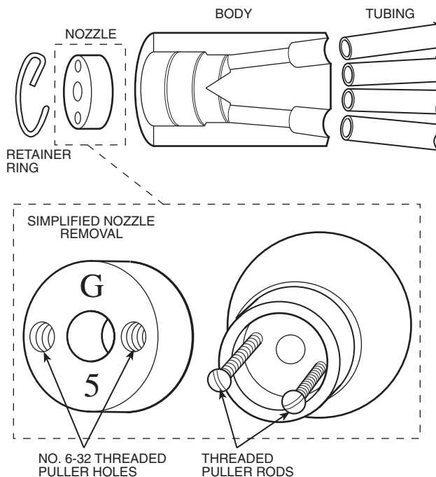
Fig. 98 — Nozzle Change-Out
