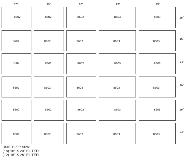
Fig. 186 — Filter Mixing Box and Angle Filter Arrangement — 2-in. or 4-in. (cont)
