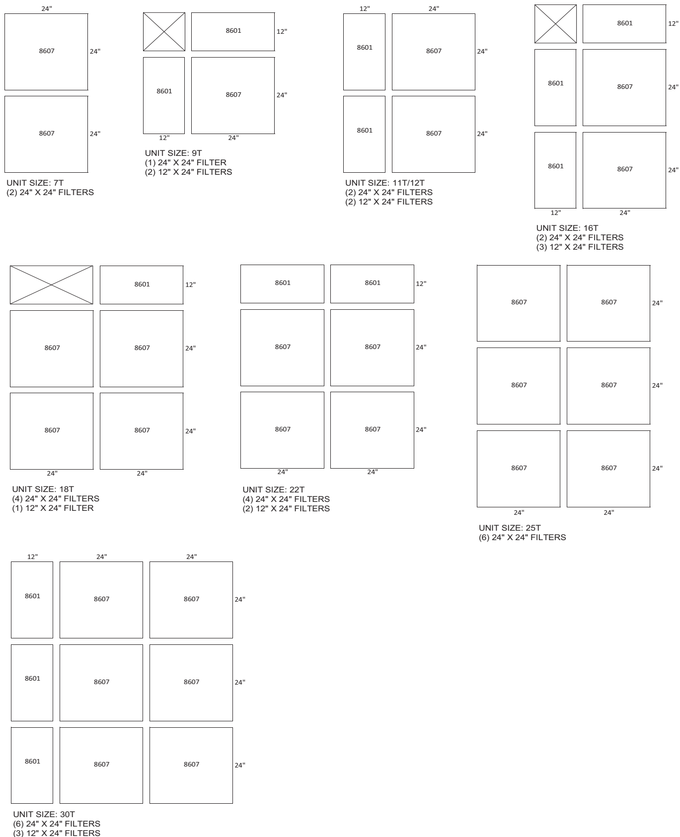
Fig. 189 — HEPA Filter Arrangement (cont)
