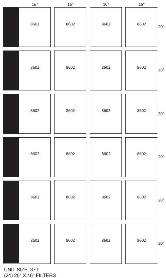
Fig. 186 — Filter Mixing Box and Angle Filter Arrangement — 2-in. or 4-in. (cont)
