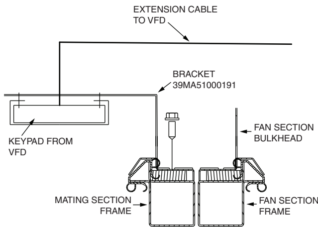
Fig. 158 — Remote Keypad Assembly Location
