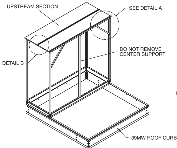
Fig. 26 — 39MW Split Assembly
