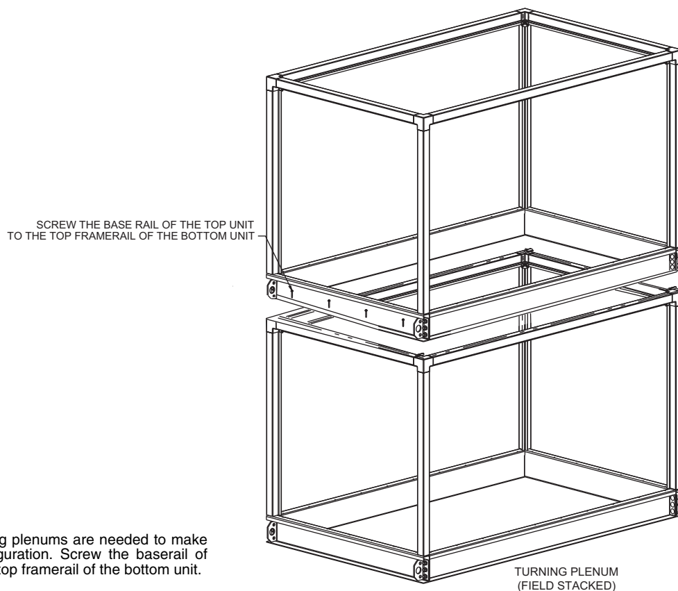
Fig. 43 — Stacked Turning Plenum
