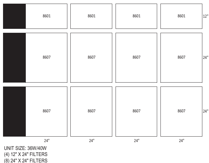
Fig. 187 — Side Load Bag/Cartridge Filter Arrangement
