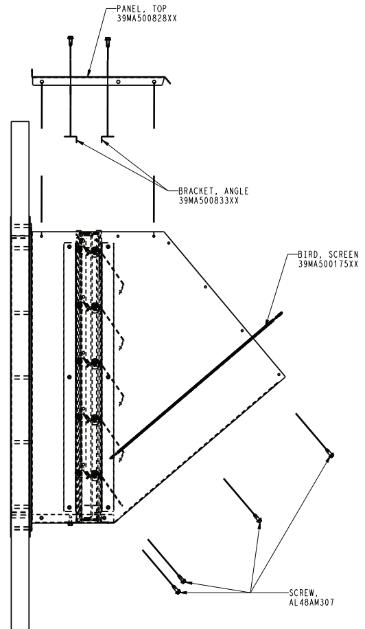
Fig. 76 — Attaching Bird Screen and Top Panel
