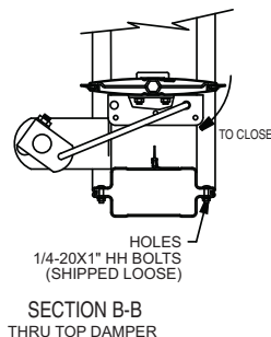
Fig. 36 — Face and Bypass Section Detail
