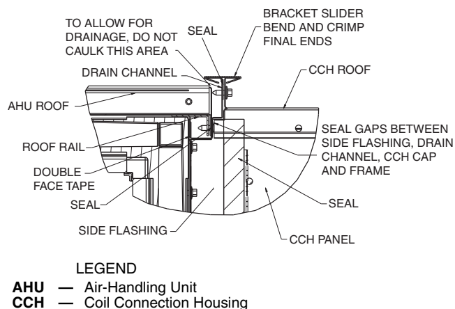
Fig. 61 — Side View
