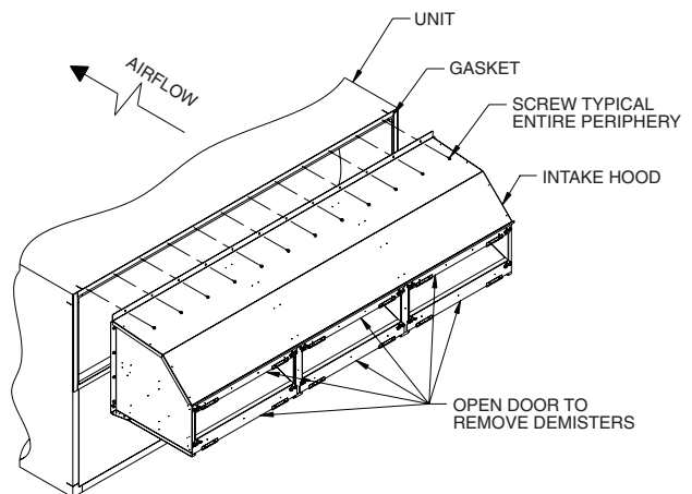
Fig. 49 — Rear Intake Hood (Size 30 Shown)
