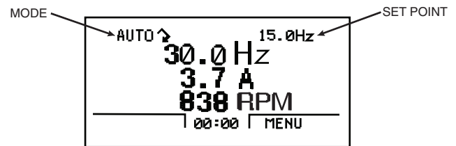
Fig. 124 — Standard Display Example
