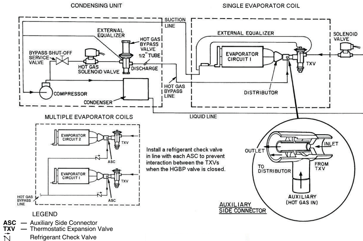
Fig. 104 — Hot Gas Bypass Piping
