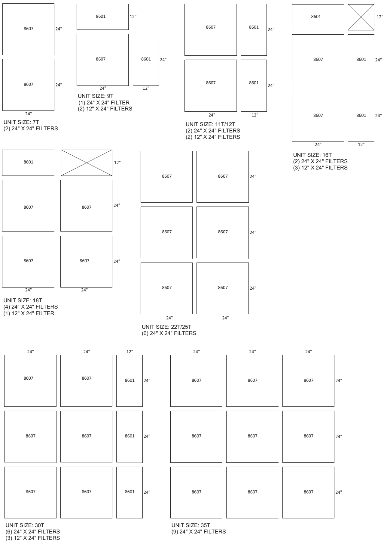
Fig. 188 — Front Load Bag/Cartridge Filter Arrangement (cont)
