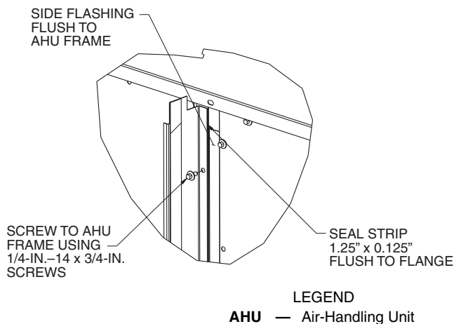
Fig. 56 — Screw the Side Flashings to Unit
