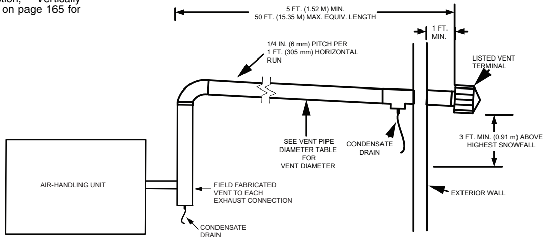
Category III Horizontal Furnace Venting (through Sidewall) (Only dedicated furnace venting permitted. Each furnace must have its own individual vent pipe and terminal.)
