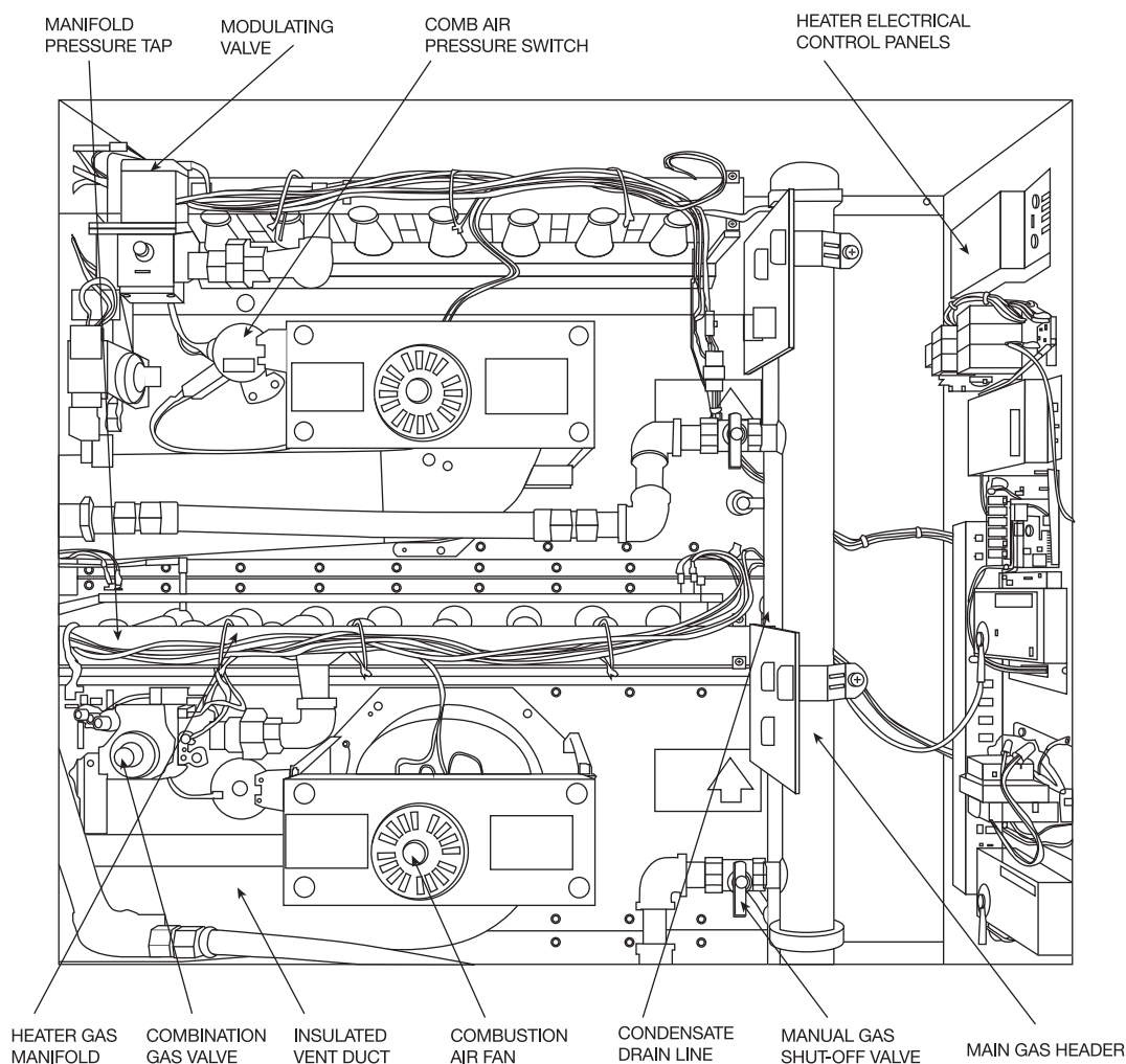
Fig. 146 — Gas-Fired Rack Furnace Components
