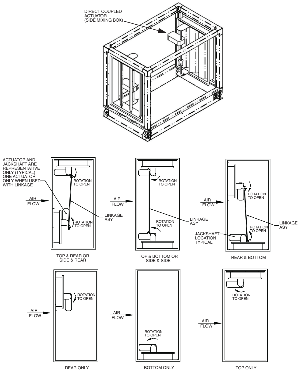
Fig. 39 — Mixing Box/Filter Mixing Box, Typical Damper Arrangements (Size 14 Shown)
