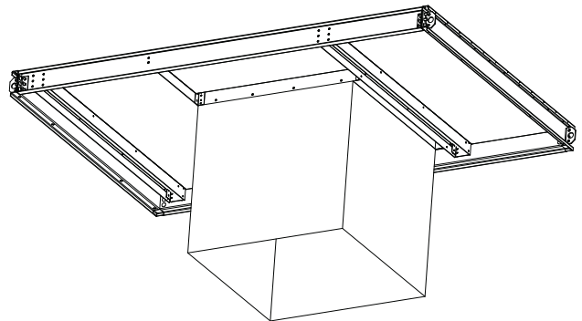
Fig. 32 — Bottom Duct Connection — Housed Fans
