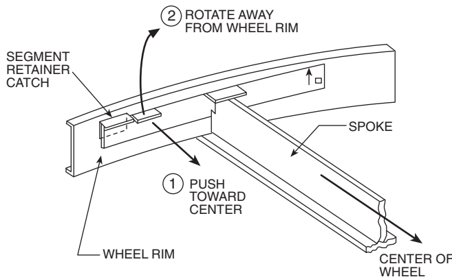
Fig. 160 — Segment Retainer
