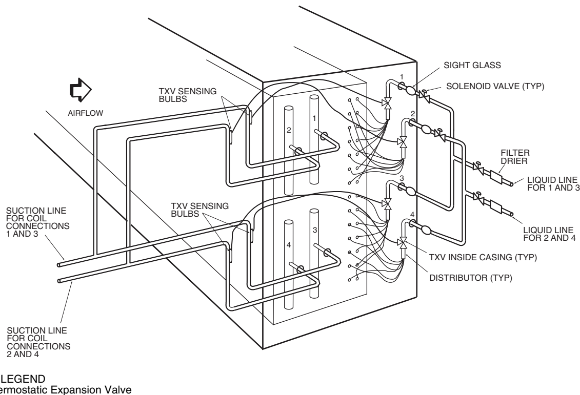
Fig. 103 — Row-Split Coil Manifolding (Typical)
