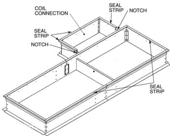
Fig. 54 — Installing Seal Strip
