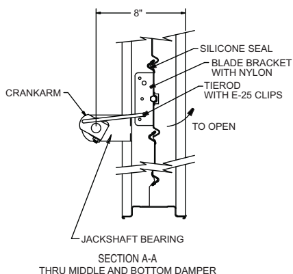
Fig. 36 — Face and Bypass Section Detail
