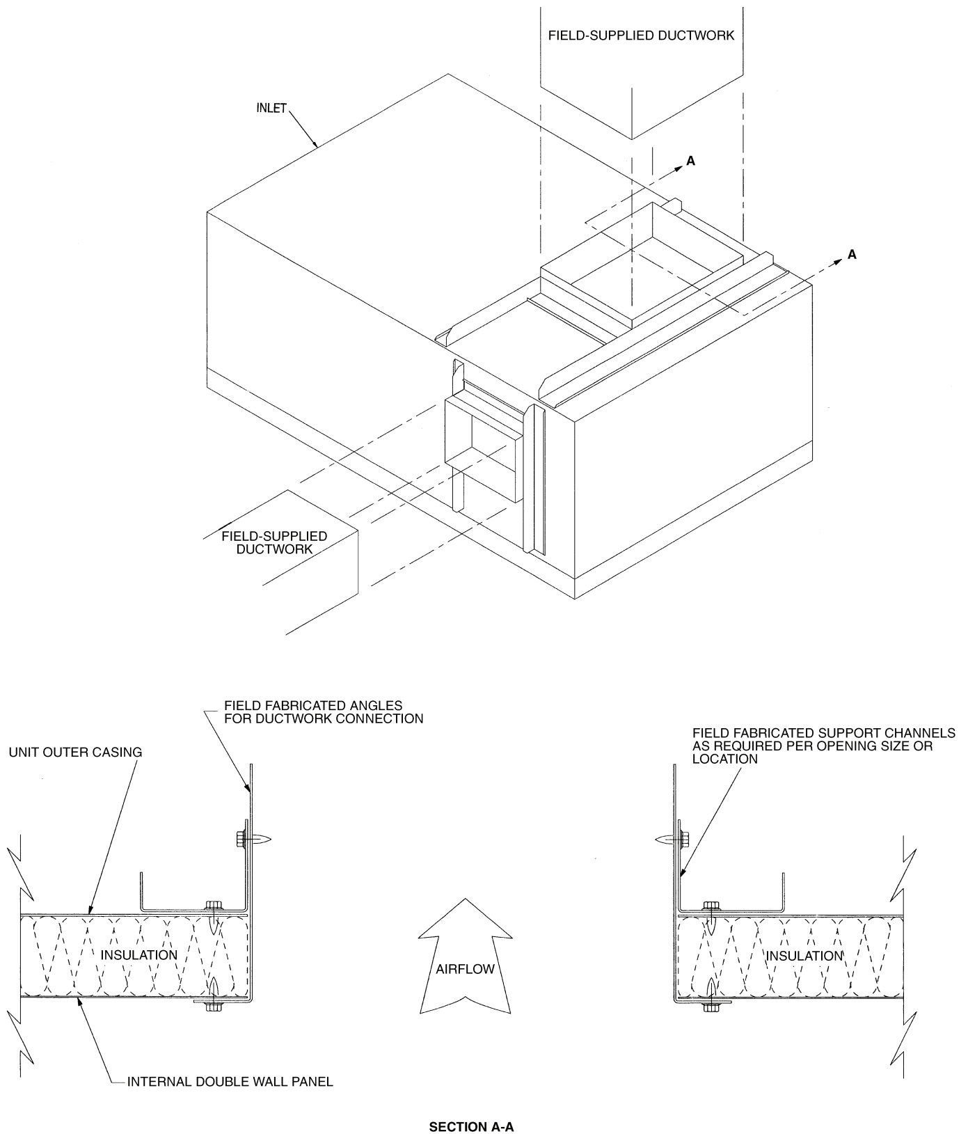
Fig. 35 — Discharge Fabrication, Draw-Thru Plenum Fans
