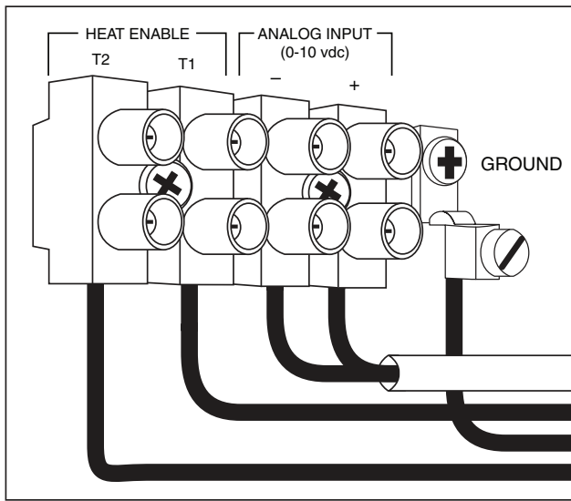
Fig. 145 — Gas-Fired Rack System Furnace Typical Wiring Diagram
