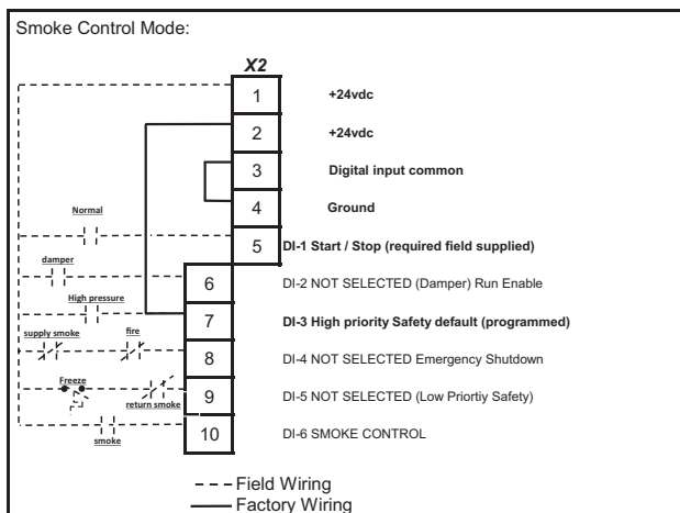
Fig. 128 — Smoke Detector Typical Wiring Diagram
