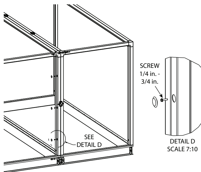
Fig. 25 — Attaching CCH at Section Split — Location of Screw Holes
