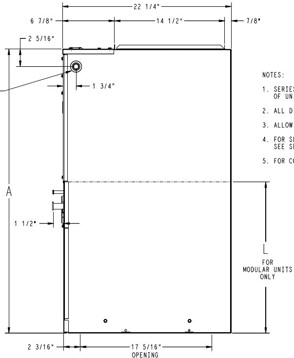
Fig. 2 – Dimensions, English, sheet 1
