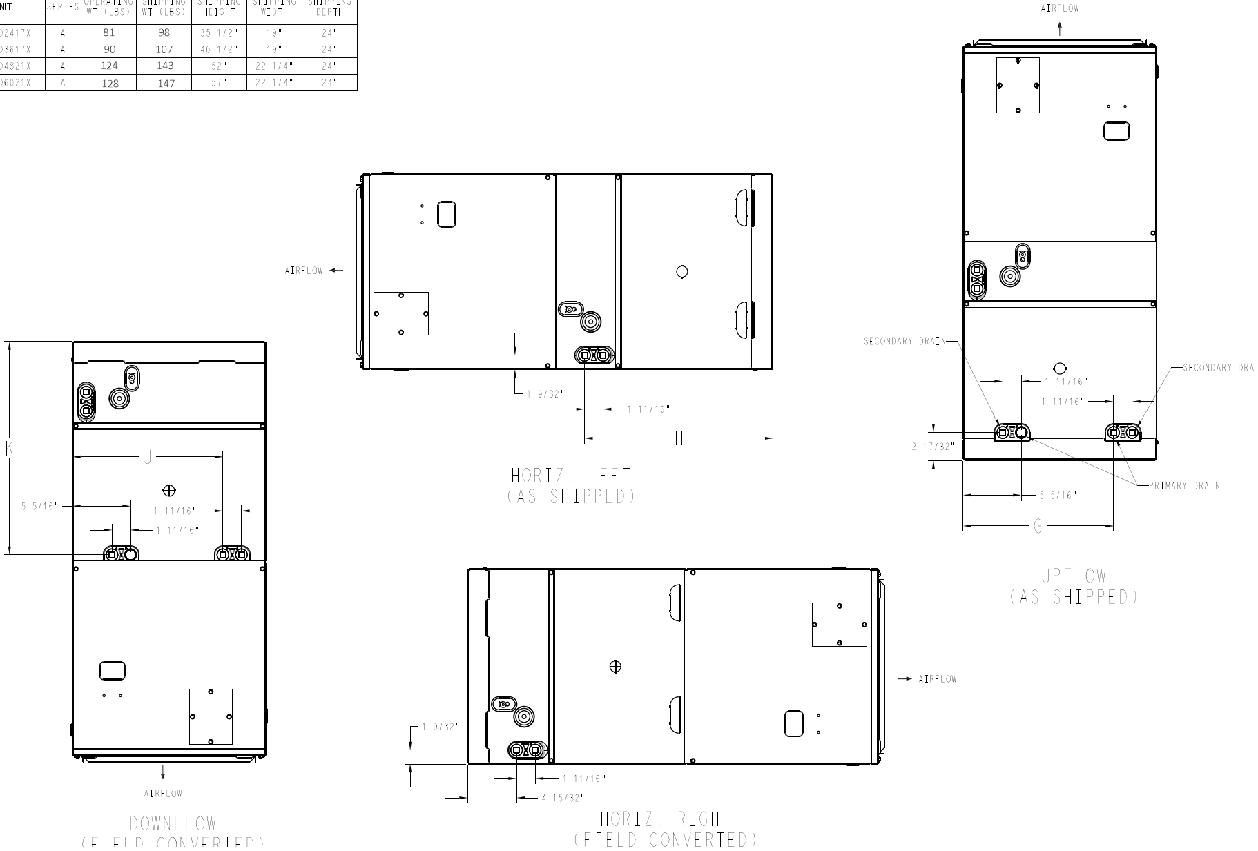
Fig. 3 – Dimensions, English, sheet 2
