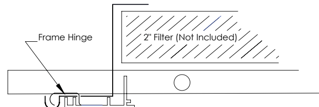
935TFG Frame Detail
