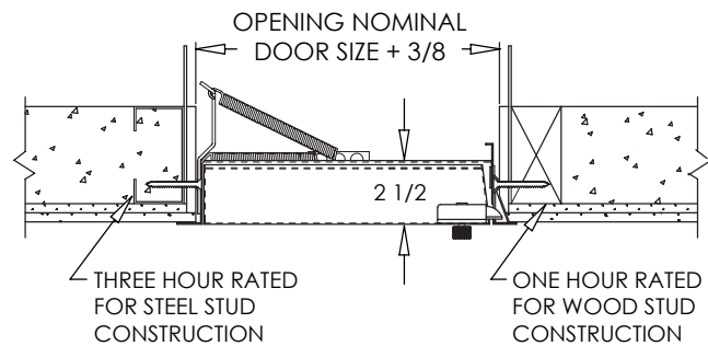
6900 CEILING OPENING
