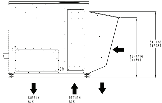
HORIZONTAL ECONOMIZER
