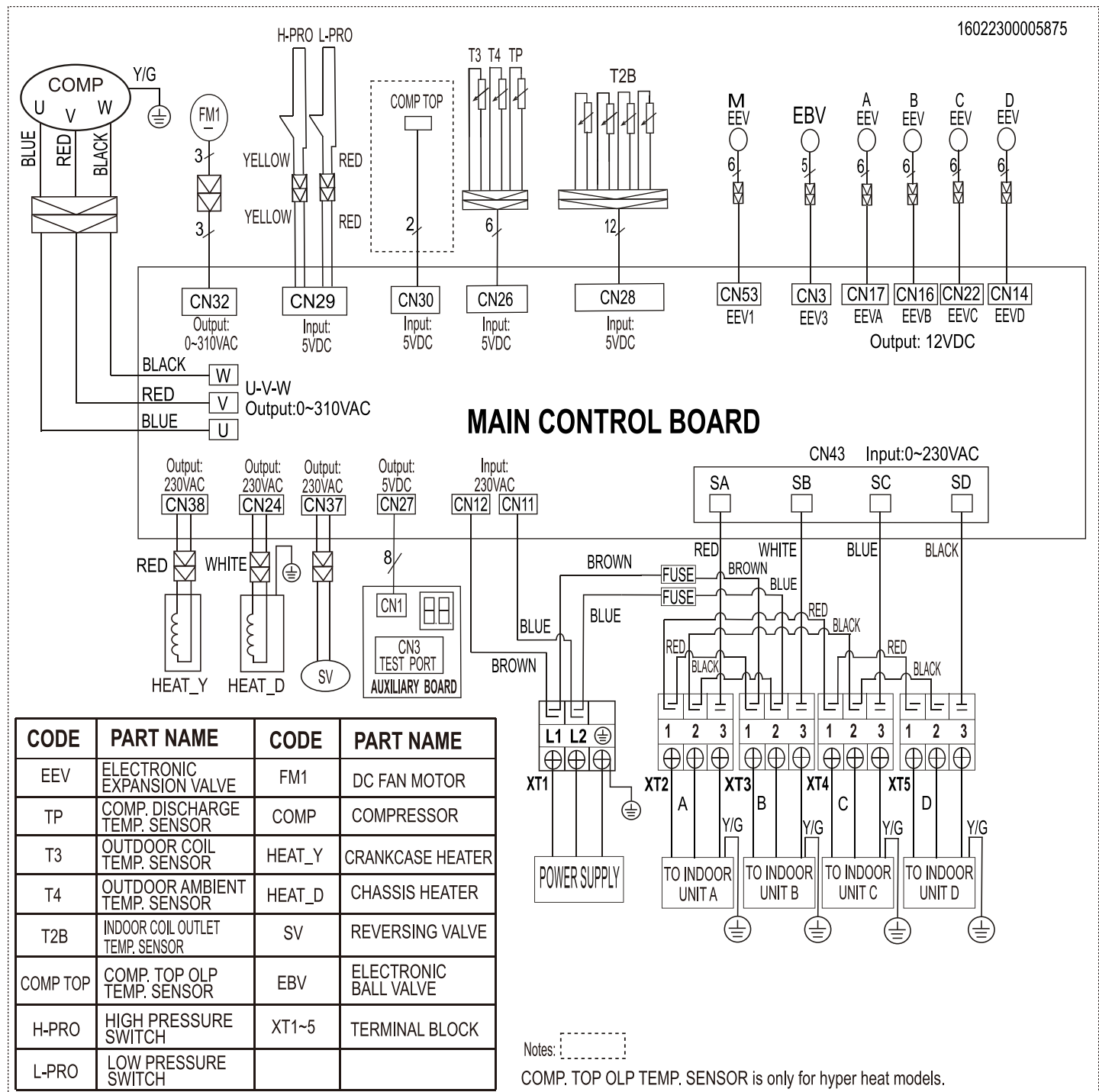
Fig. 14 — Wiring Diagram 24K
