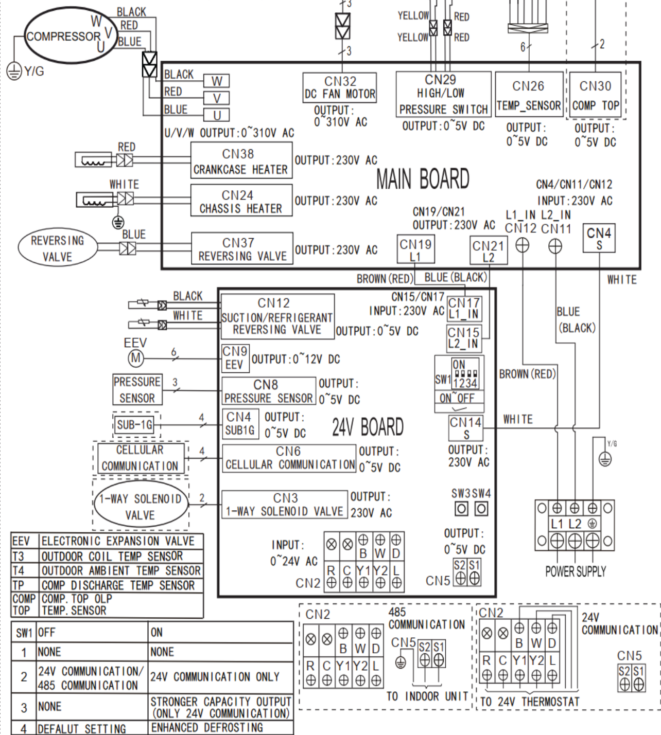
Fig. 38 — Wiring Diagram Size 30K
