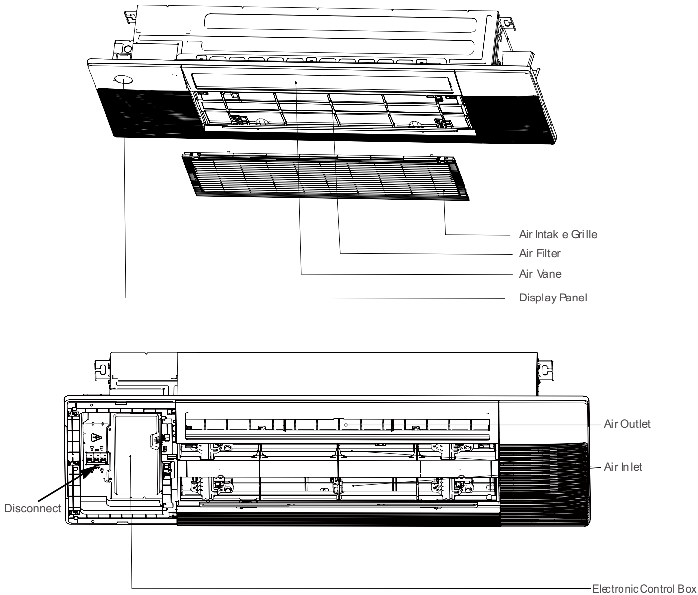
Fig. 12 – Part Names
