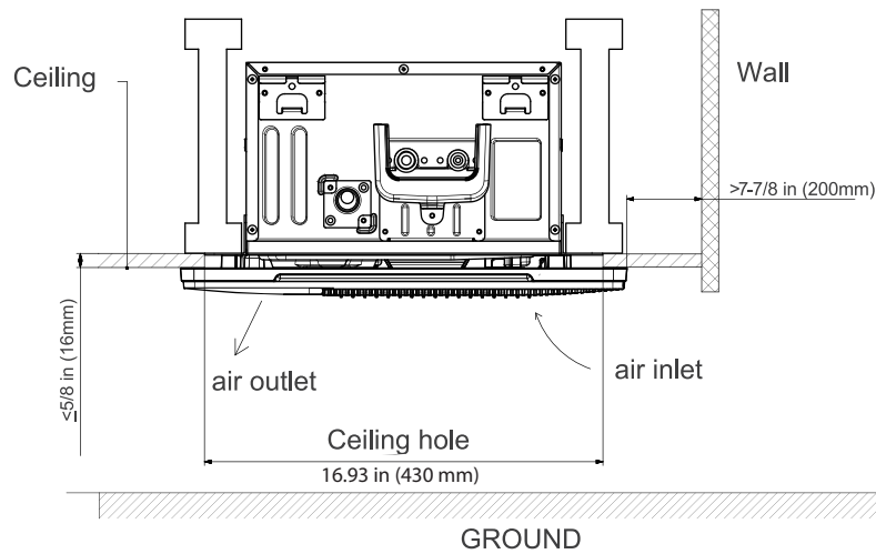
Fig. 11 – Clearance
