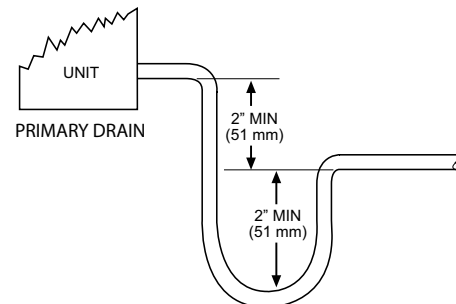
Fig. 11 – Recommended Condensate Trap
