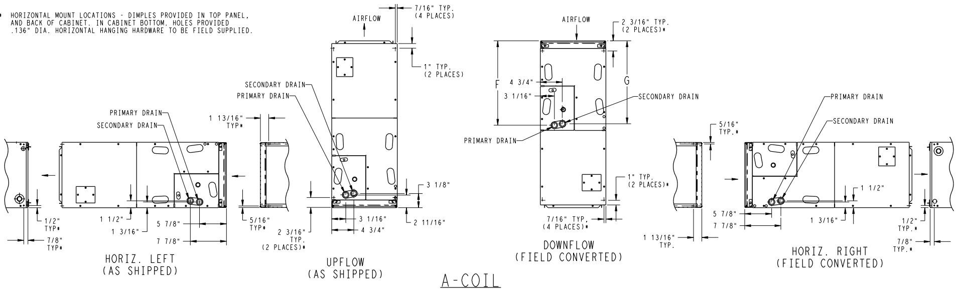
Fig. 2 – Dimensions, sheet 2
