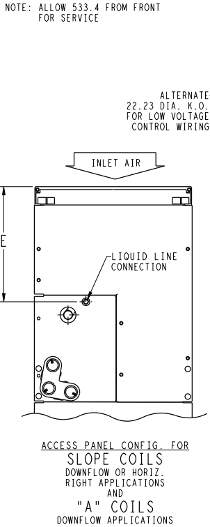
Fig. 3 – Dimensions, sheet 3
