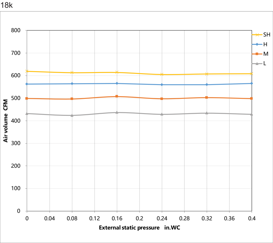
Fig. 22 – Low Static Pressure Curves – Constant Air Volume
