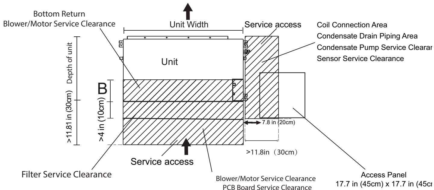
Fig. 9 – Maintenance Clearance
