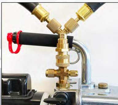
Increase speed of evacuation with the Y-FORCE Dual, High-speed Coupler Connector and two large diameter hoses.
