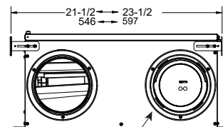
MOTORIZED DAMPER
