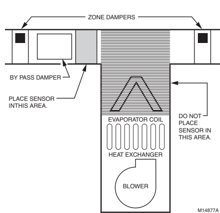
Fig. 2. DATS mounting location.
