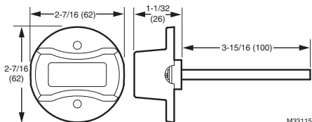
Fig. 1. C7735A dimensions in in. (mm).
